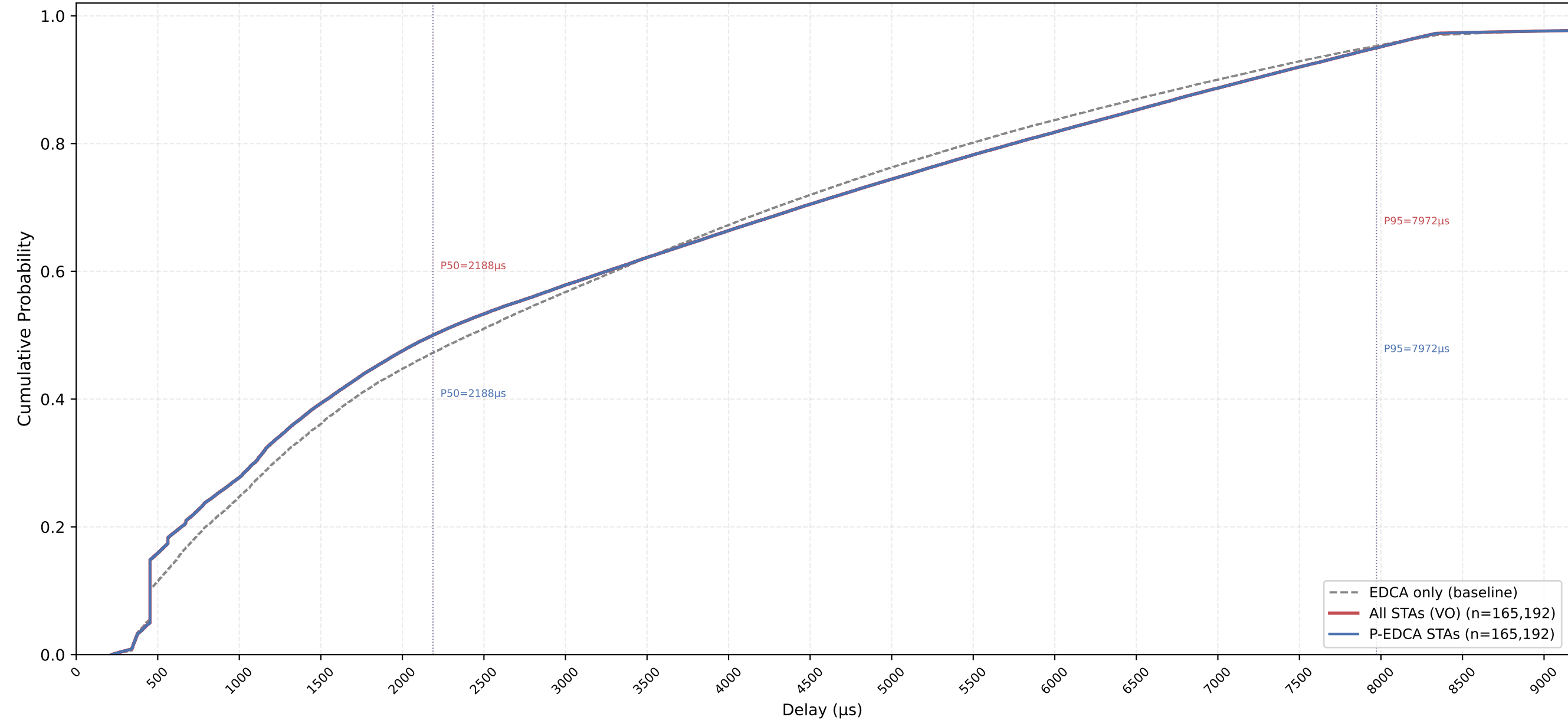
VO Delay CDF — P-EDCA / Legacy / All | CWds=1 × QSRC=4 × PSRC=3 nSta=30, nPedca=30/30, 1Mbps, avg of 10 runs
