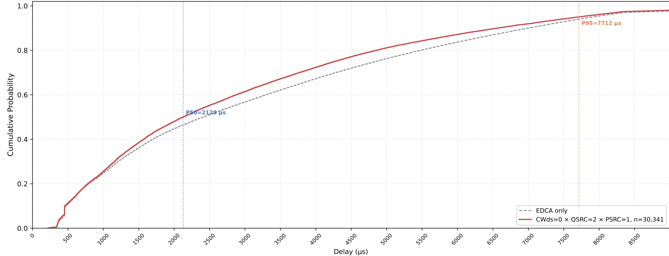
P-EDCA STA VO Delay CDF — CWds=0 × QSRC=2 × PSRC=1 nSta=30, nPedca=5, 1Mbps, avg of 10 runs
