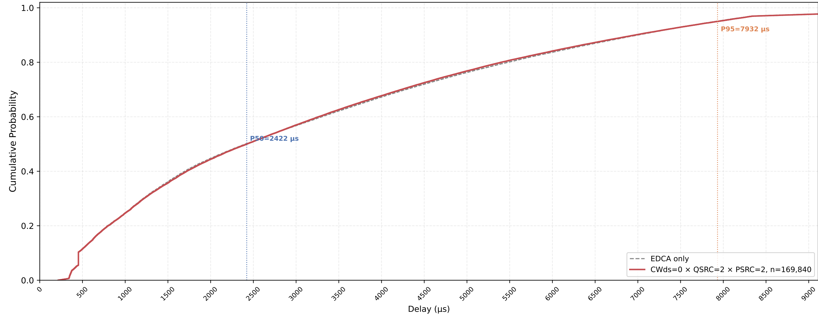
VO (all STAs) Delay CDF — CWds=0 × QSRC=2 × PSRC=2 nSta=30, nPedca=5, 1Mbps, avg of 10 runs
