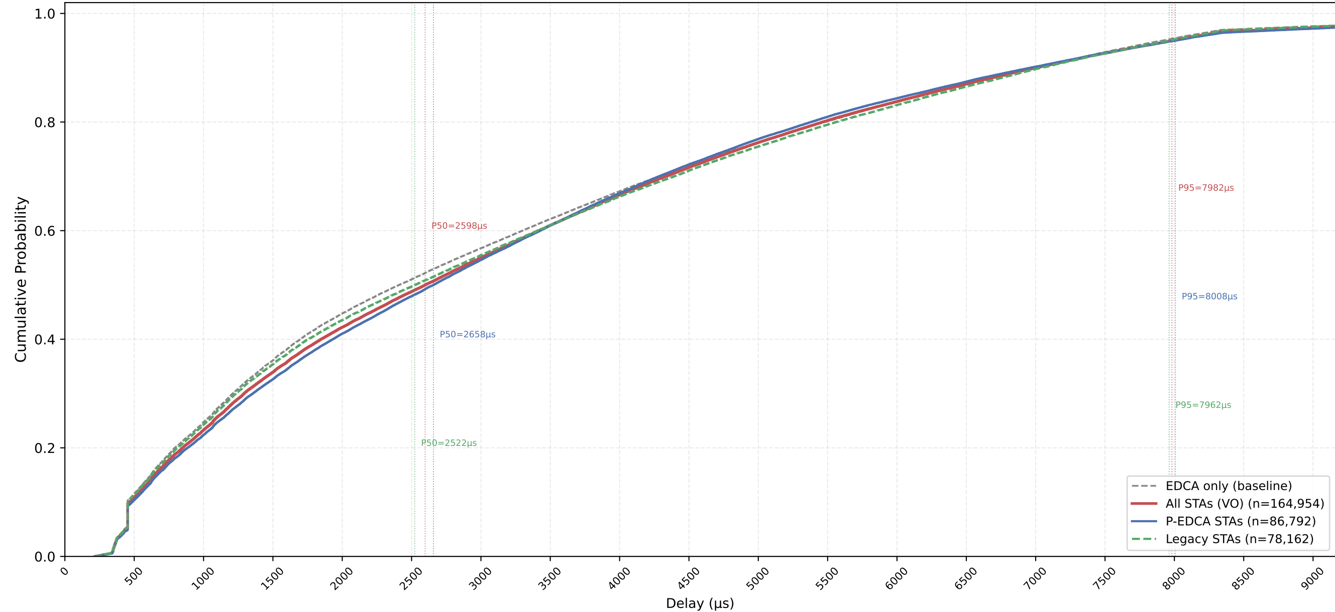
VO Delay CDF — P-EDCA / Legacy / All | CWds=0 × QSRC=2 × PSRC=3 nSta=30, nPedca=15/30, 1Mbps, avg of 10 runs
