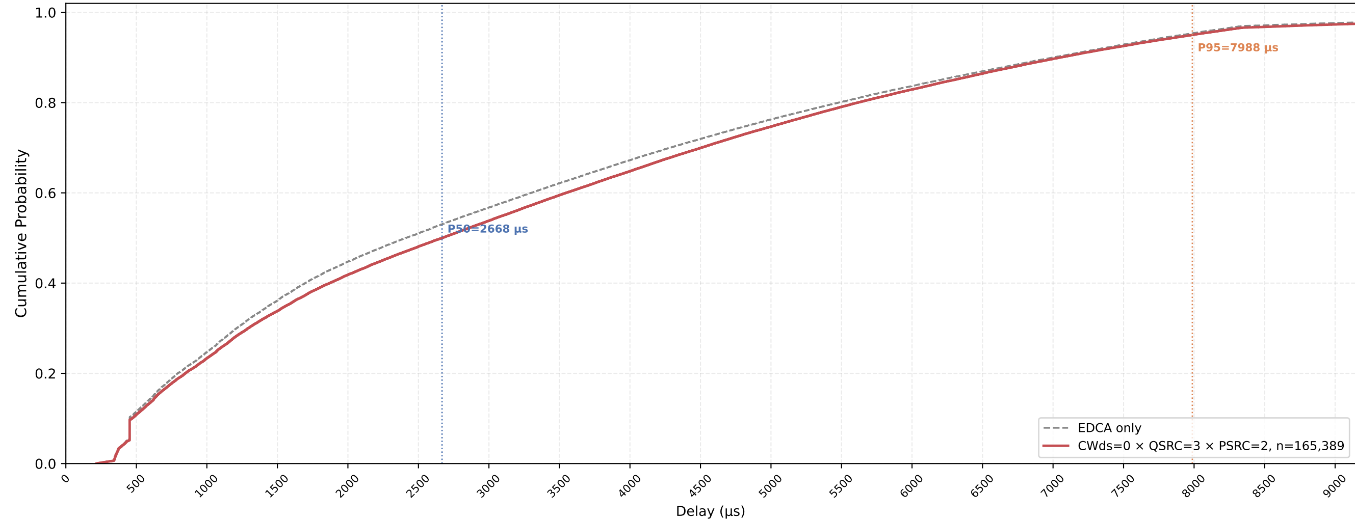
P-EDCA STA VO Delay CDF — CWds=0 × QSRC=3 × PSRC=2 nSta=30, nPedca=30, 1Mbps, avg of 10 runs
