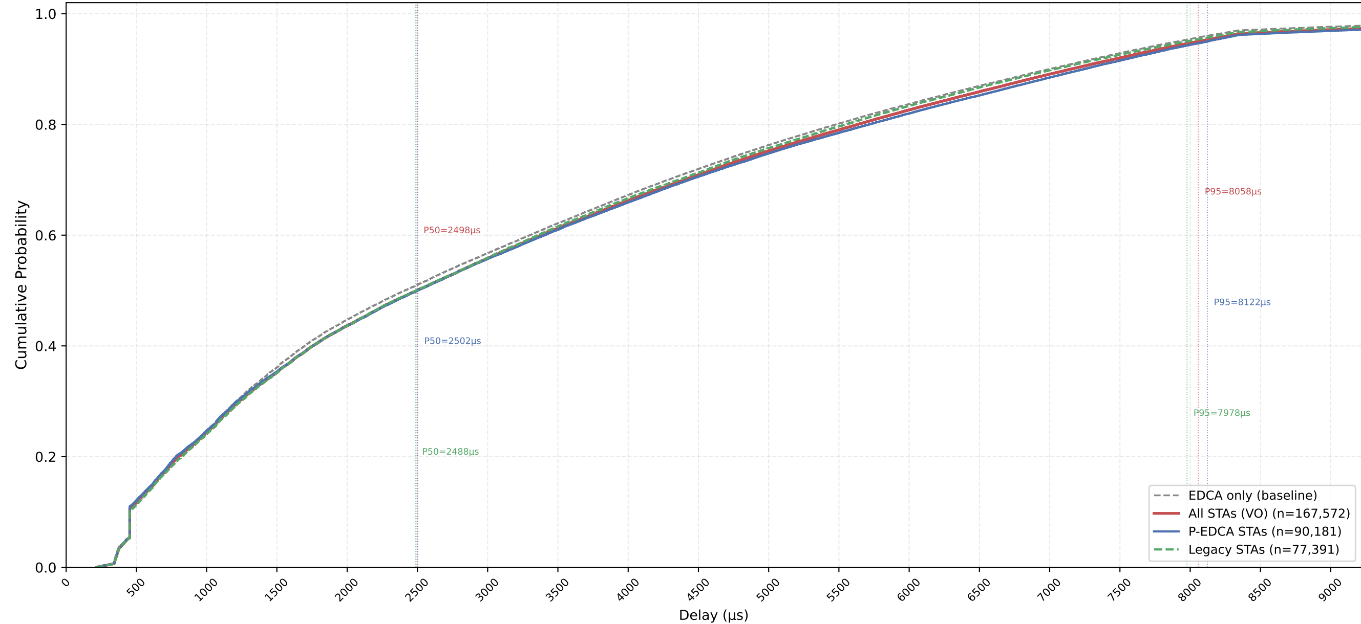
VO Delay CDF — P-EDCA / Legacy / All | CWds=0 × QSRC=5 × PSRC=3 nSta=30, nPedca=15/30, 1Mbps, avg of 10 runs
