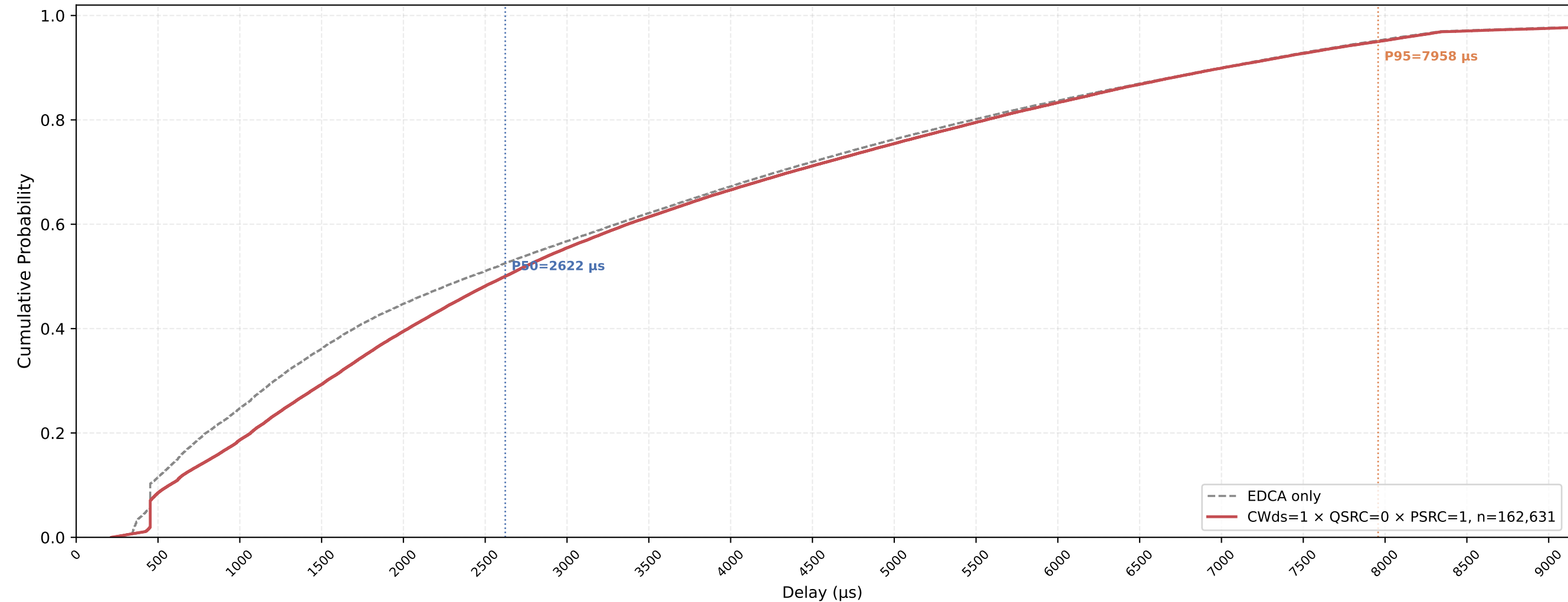
VO (all STAs) Delay CDF — CWds=1 × QSRC=0 × PSRC=1 nSta=30, nPedca=30, 1Mbps, avg of 10 runs
