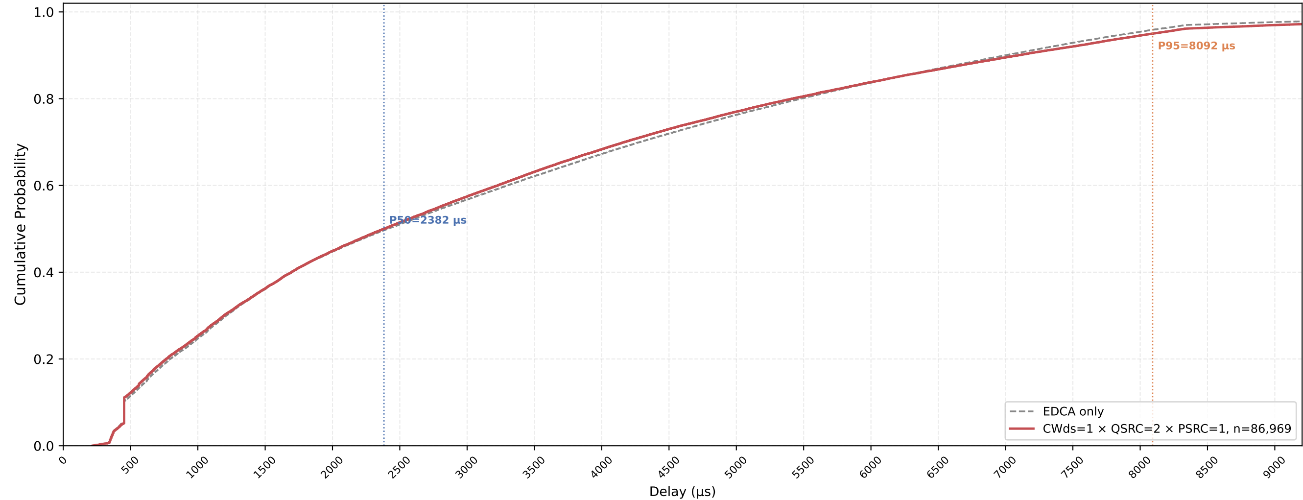
P-EDCA STA VO Delay CDF — CWds=1 × QSRC=2 × PSRC=1 nSta=30, nPedca=15, 1Mbps, avg of 10 runs
