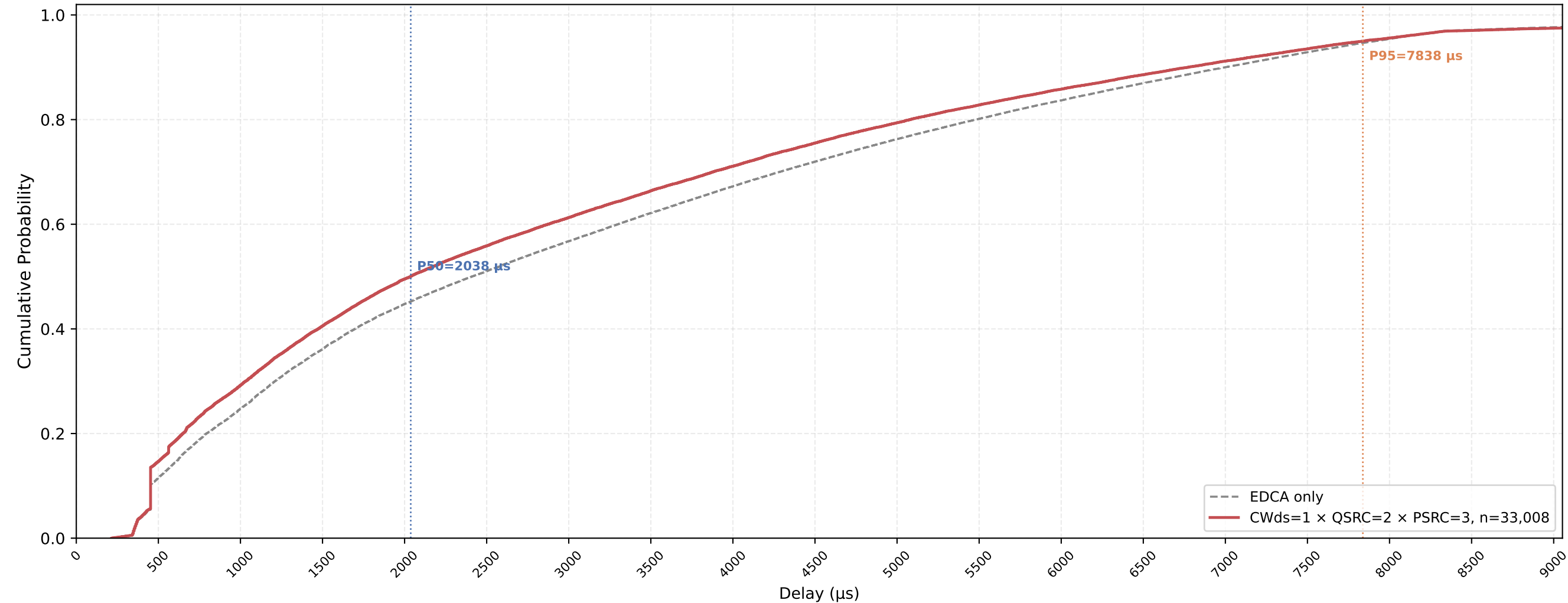
P-EDCA STA VO Delay CDF — CWds=1 × QSRC=2 × PSRC=3 nSta=30, nPedca=5, 1Mbps, avg of 10 runs
