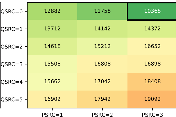
P-EDCA STA VO Delay — P99 Dual-DS (2x DS-CTS) (nSta=30, 1Mbps, black box = best in panel) colour scale 7632-24542 shared across mono-DS & dual-DS — panels are directly comparable
