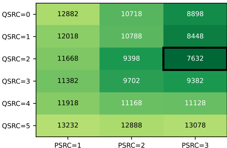
P-EDCA STA VO Delay — P99 Dual-DS (2x DS-CTS) (nSta=30, 1Mbps, black box = best in panel) colour scale 7632-24542 shared across mono-DS & dual-DS — panels are directly comparable
