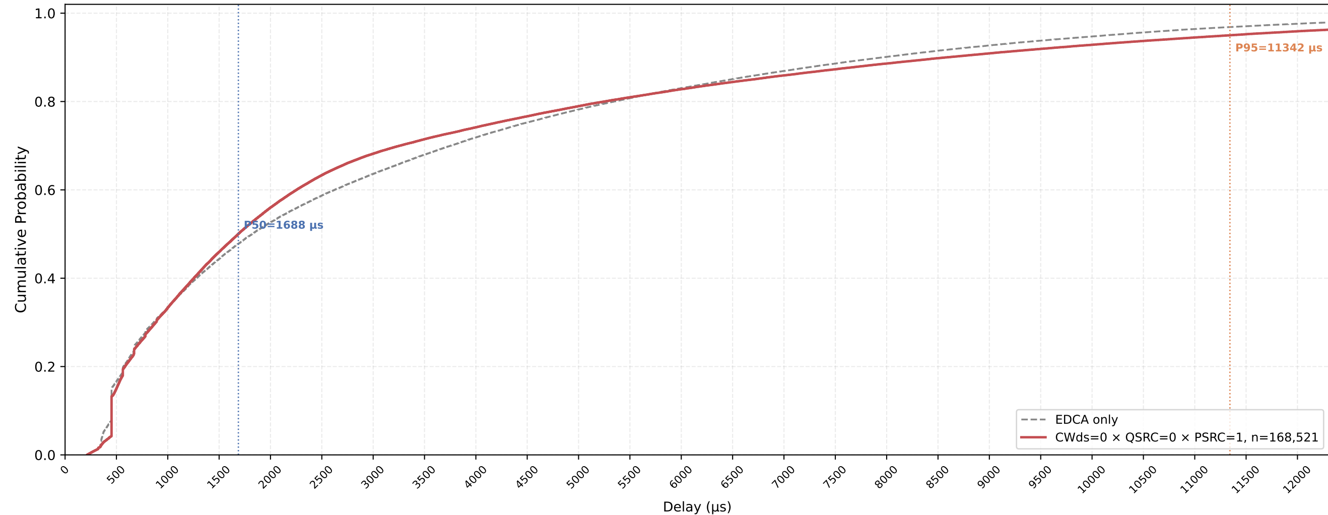
VO (all STAs) Delay CDF — CWds=0 × QSRC=0 × PSRC=1 nSta=30, nPedca=15, 1Mbps, avg of 10 runs
