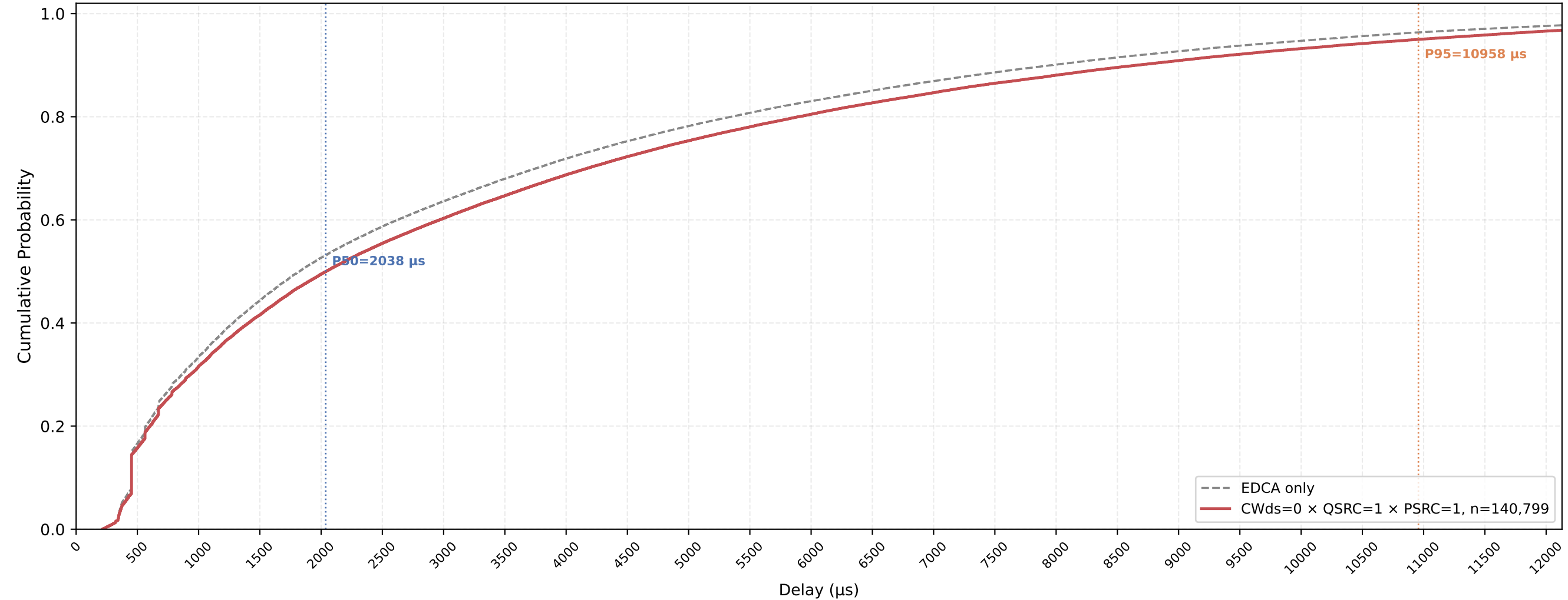
Legacy STA VO Delay CDF — CWds=0 × QSRC=1 × PSRC=1 nSta=30, nPedca=5, 1Mbps, avg of 10 runs
