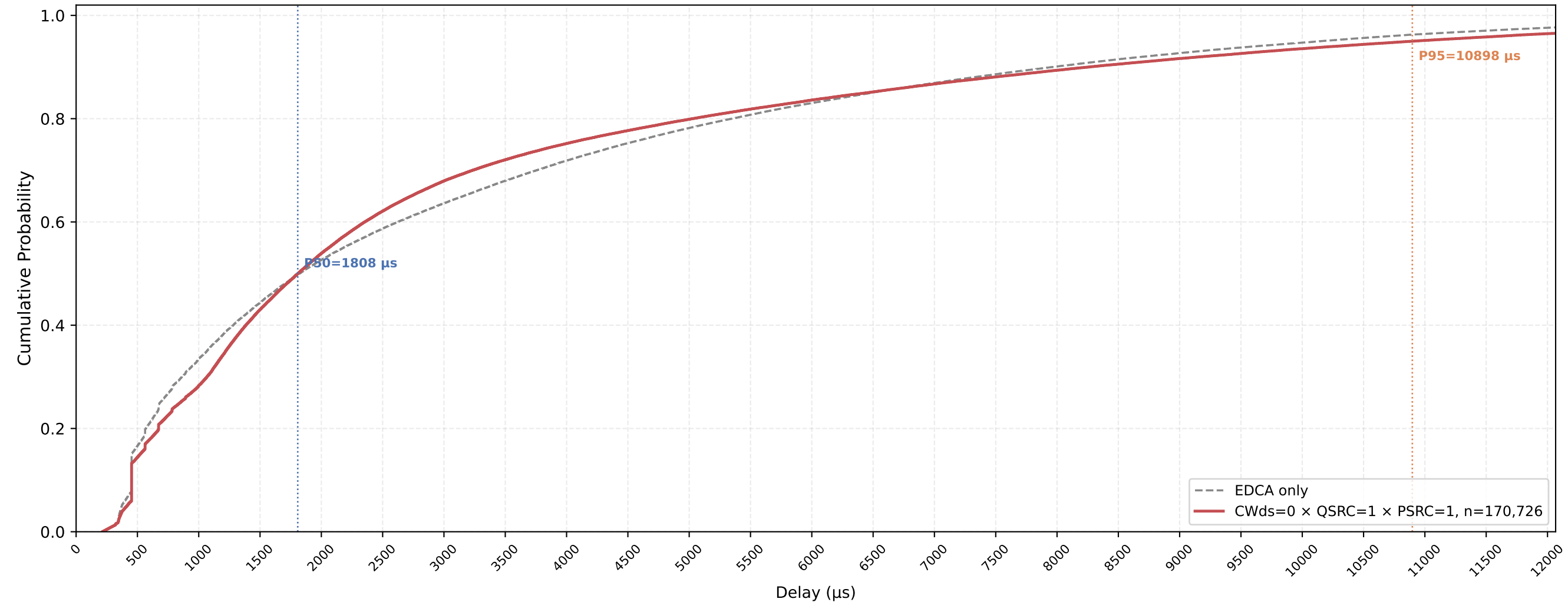
VO (all STAs) Delay CDF — CWds=0 × QSRC=1 × PSRC=1 nSta=30, nPedca=15, 1Mbps, avg of 10 runs
