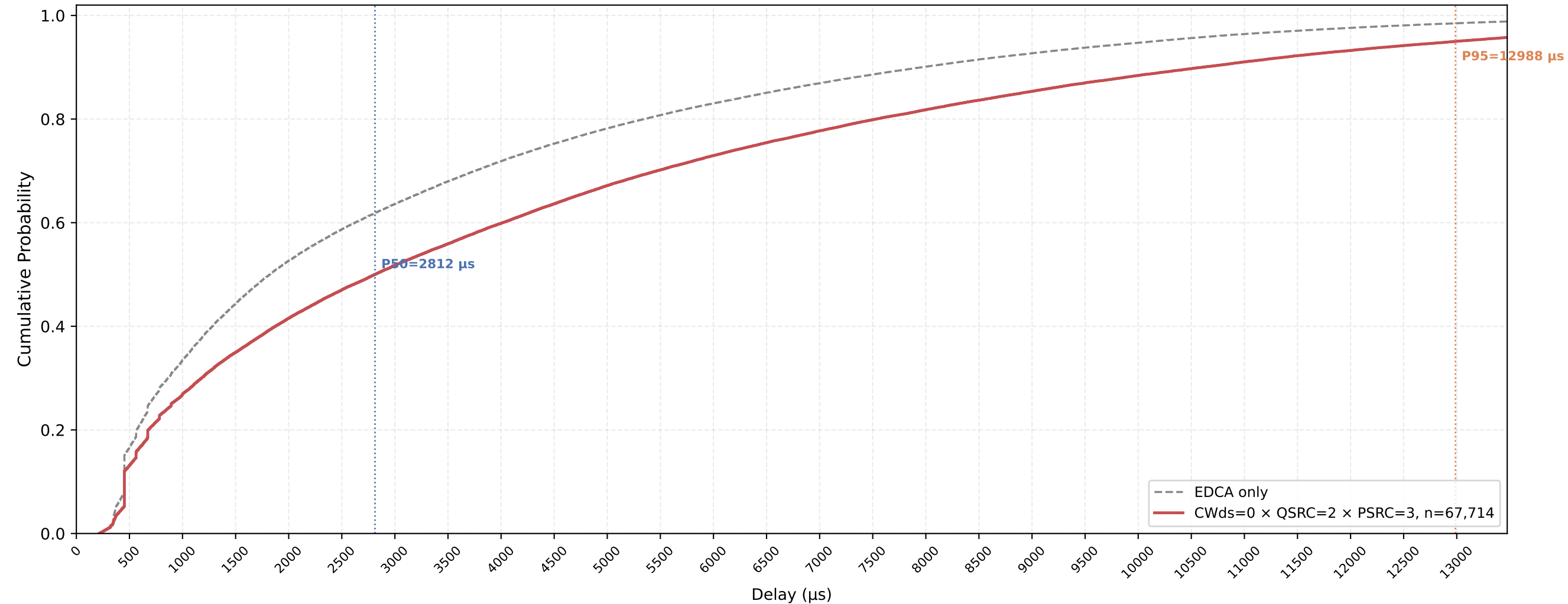
Legacy STA VO Delay CDF — CWds=0 × QSRC=2 × PSRC=3 nSta=30, nPedca=15, 1Mbps, avg of 10 runs
