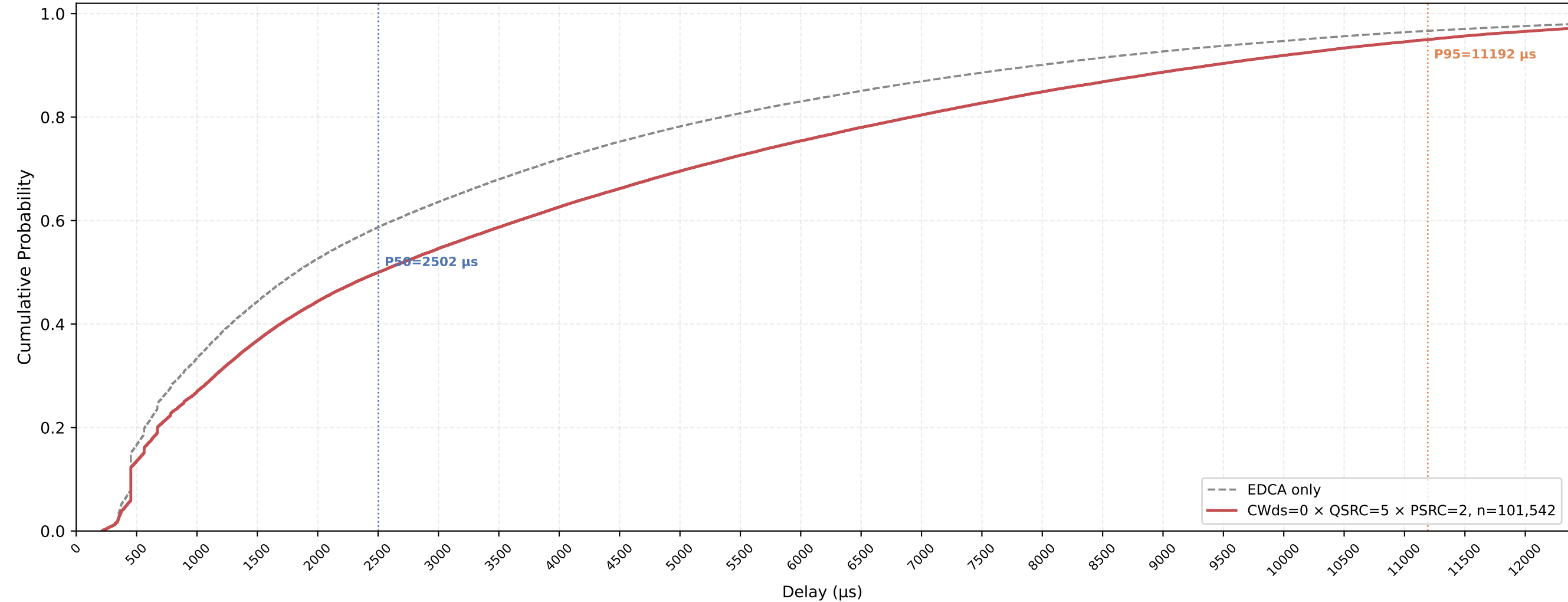
P-EDCA STA VO Delay CDF — CWds=0 × QSRC=5 × PSRC=2 nSta=30, nPedca=15, 1Mbps, avg of 10 runs
