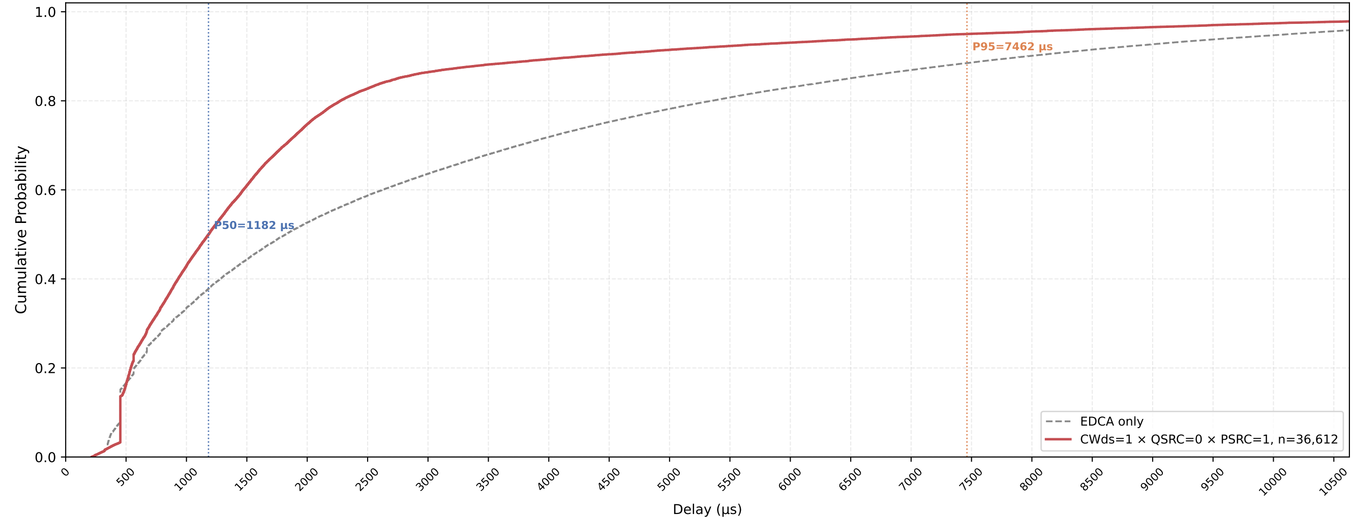
P-EDCA STA VO Delay CDF — CWds=1 × QSRC=0 × PSRC=1 nSta=30, nPedca=5, 1Mbps, avg of 10 runs
