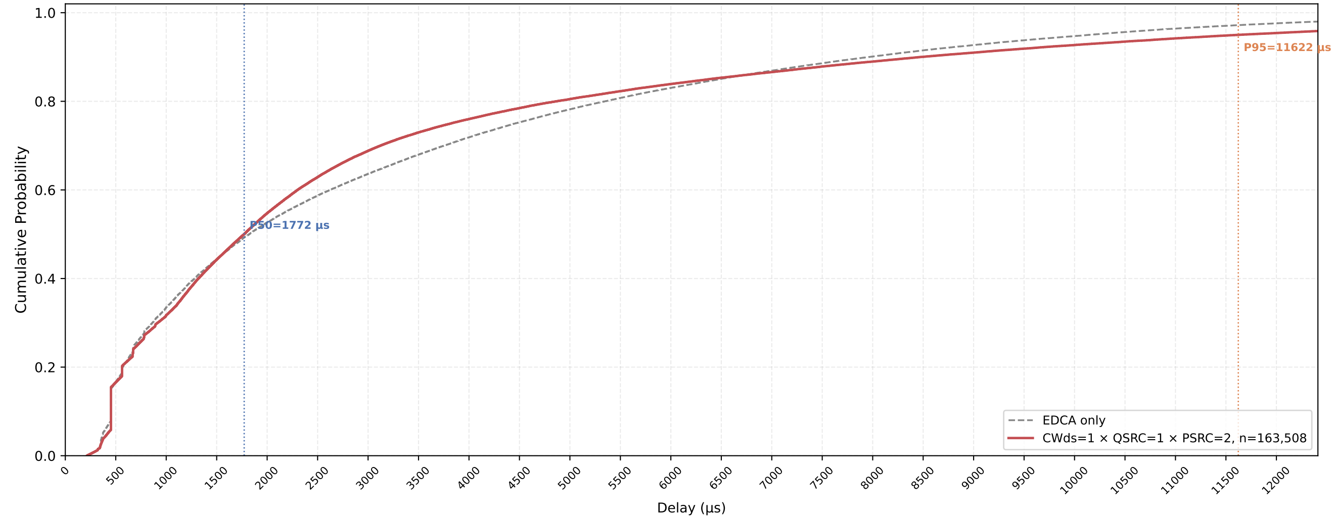
VO (all STAs) Delay CDF — CWds=1 × QSRC=1 × PSRC=2 nSta=30, nPedca=30, 1Mbps, avg of 10 runs
