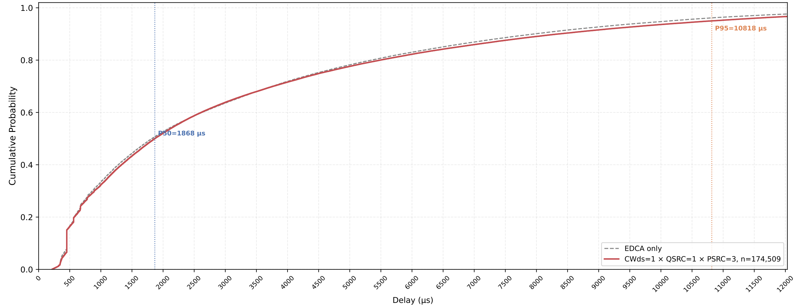
VO (all STAs) Delay CDF — CWds=1 × QSRC=1 × PSRC=3 nSta=30, nPedca=5, 1Mbps, avg of 10 runs
