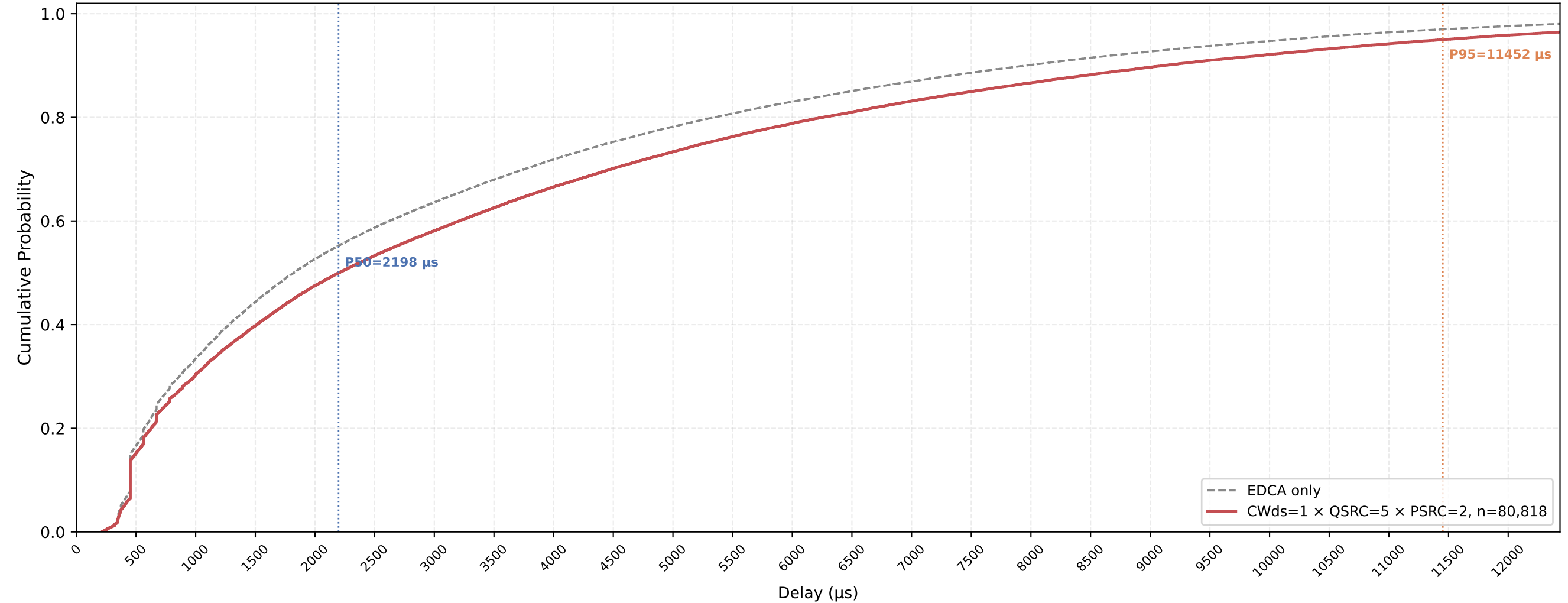
Legacy STA VO Delay CDF — CWds=1 × QSRC=5 × PSRC=2 nSta=30, nPedca=15, 1Mbps, avg of 10 runs
