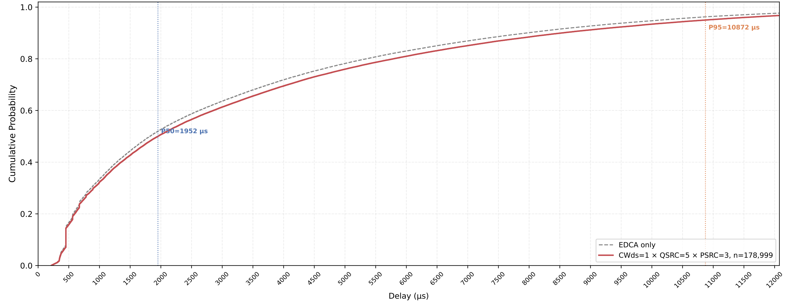
VO (all STAs) Delay CDF — CWds=1 × QSRC=5 × PSRC=3 nSta=30, nPedca=5, 1Mbps, avg of 10 runs
