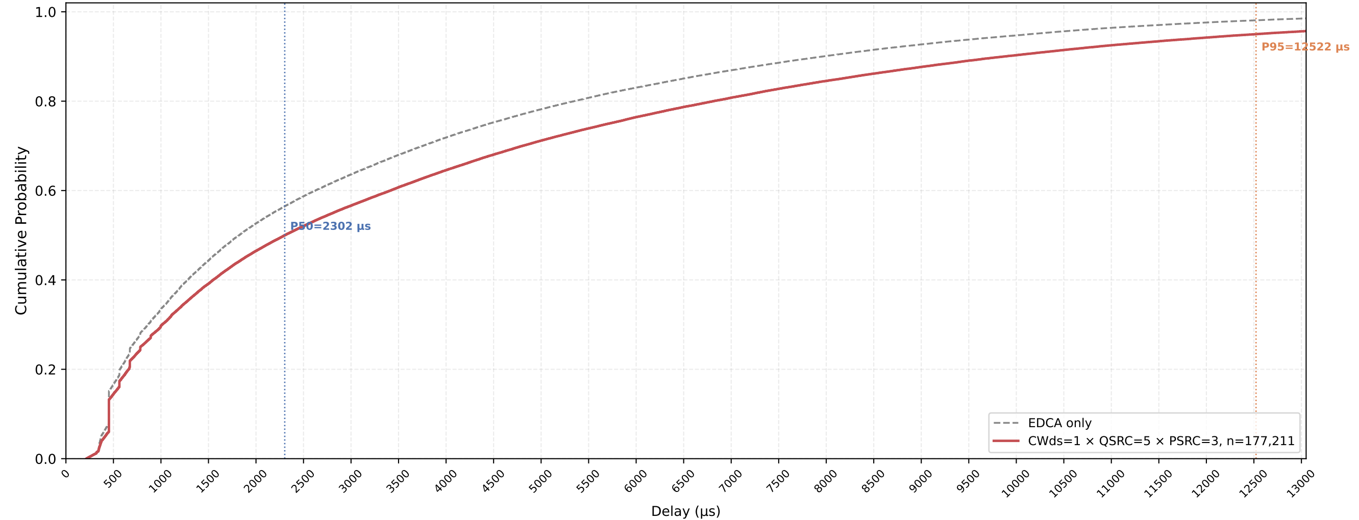
VO (all STAs) Delay CDF — CWds=1 × QSRC=5 × PSRC=3 nSta=30, nPedca=15, 1Mbps, avg of 10 runs
