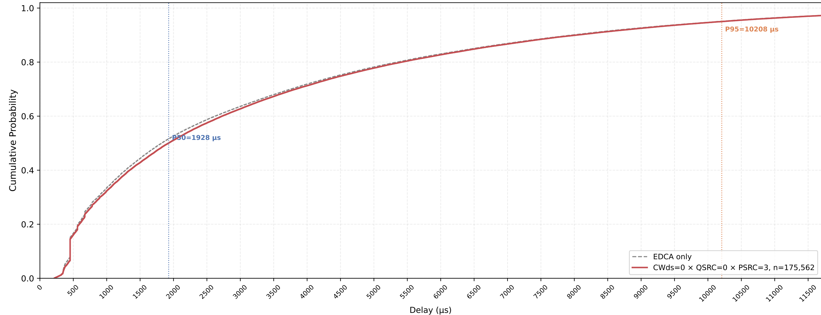
VO (all STAs) Delay CDF — CWds=0 × QSRC=0 × PSRC=3 nSta=30, nPedca=5, 1Mbps, avg of 10 runs
