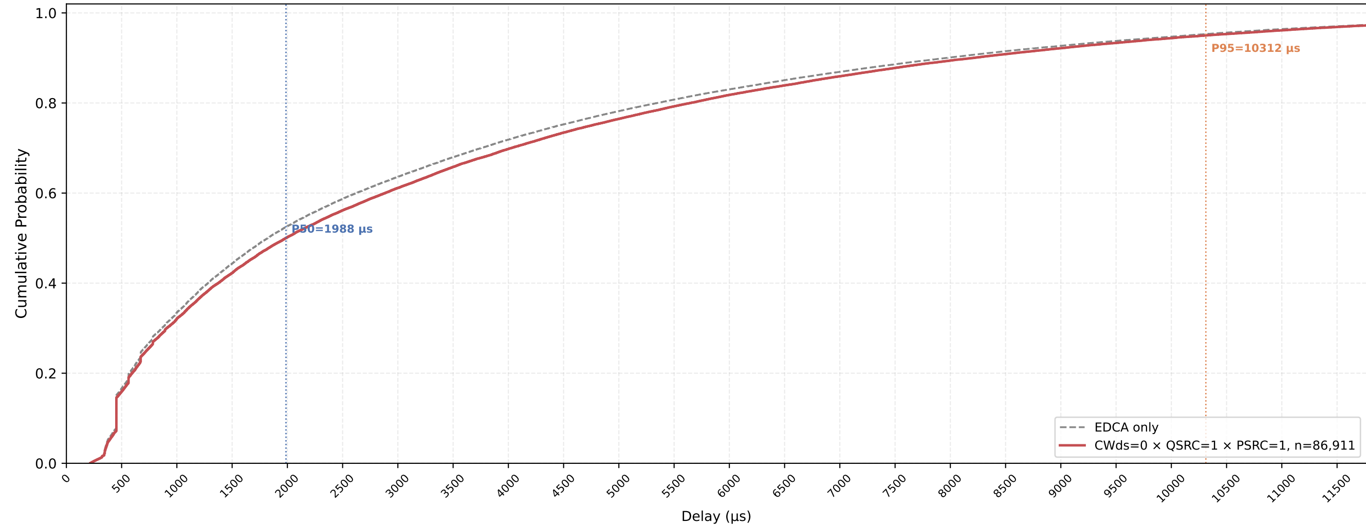
Legacy STA VO Delay CDF — CWds=0 × QSRC=1 × PSRC=1 nSta=30, nPedca=15, 1Mbps, avg of 10 runs
