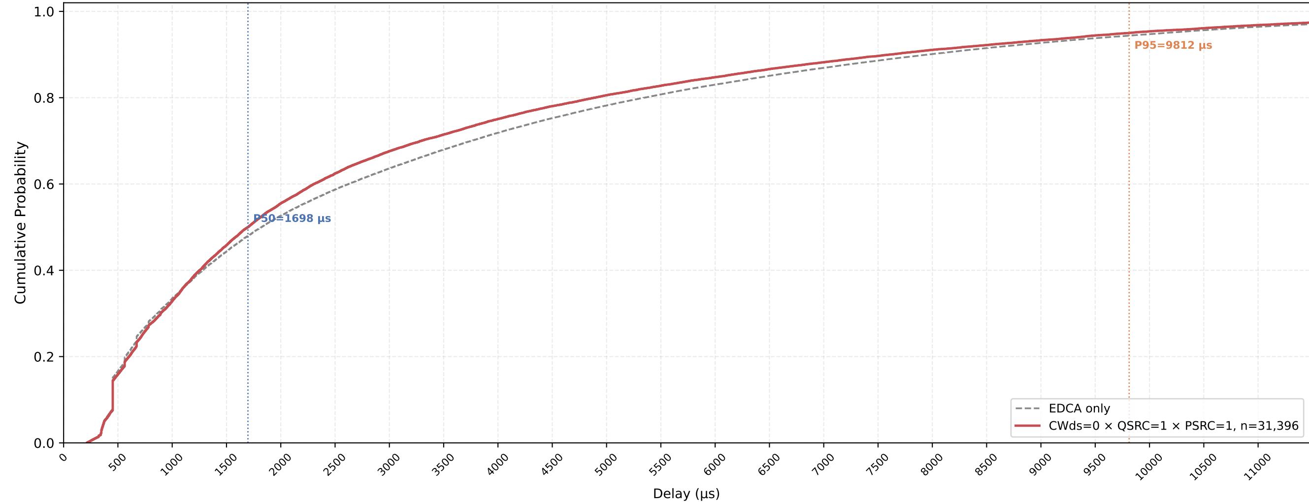
P-EDCA STA VO Delay CDF — CWds=0 × QSRC=1 × PSRC=1 nSta=30, nPedca=5, 1Mbps, avg of 10 runs
