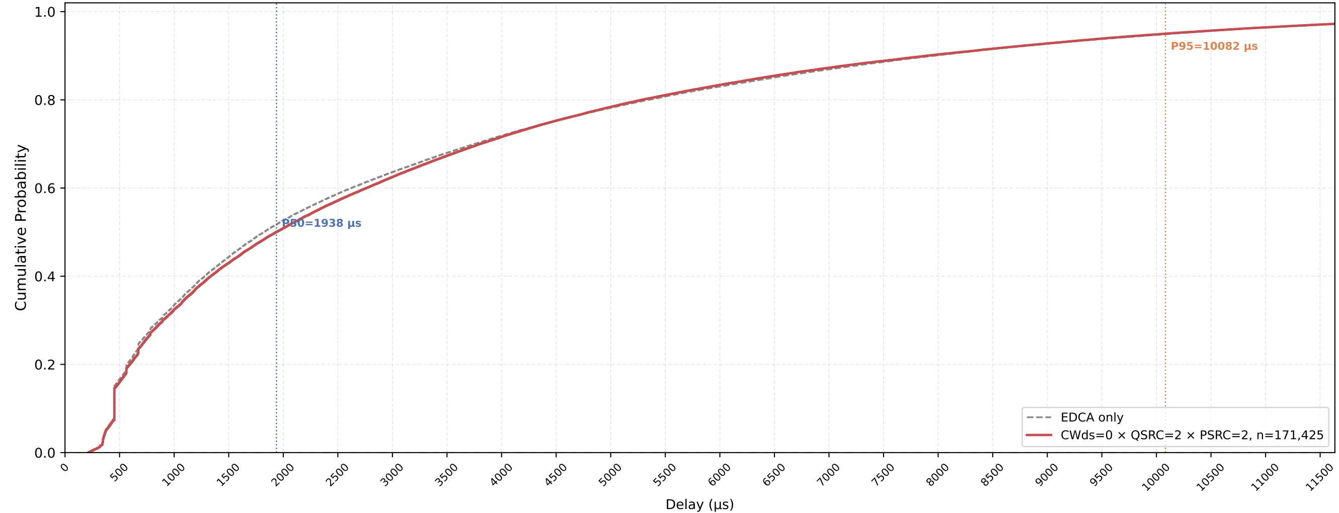
P-EDCA STA VO Delay CDF — CWds=0 × QSRC=2 × PSRC=2 nSta=30, nPedca=30, 1Mbps, avg of 10 runs
