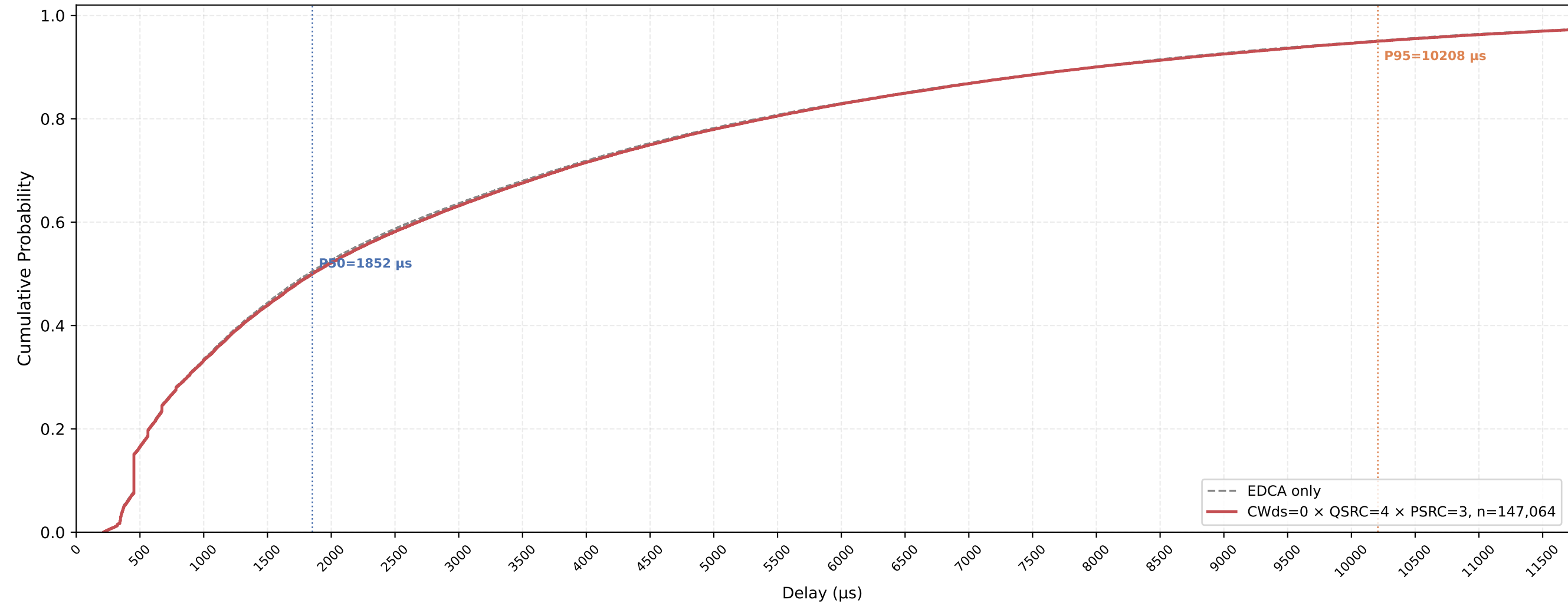
Legacy STA VO Delay CDF — CWds=0 × QSRC=4 × PSRC=3 nSta=30, nPedca=5, 1Mbps, avg of 10 runs
