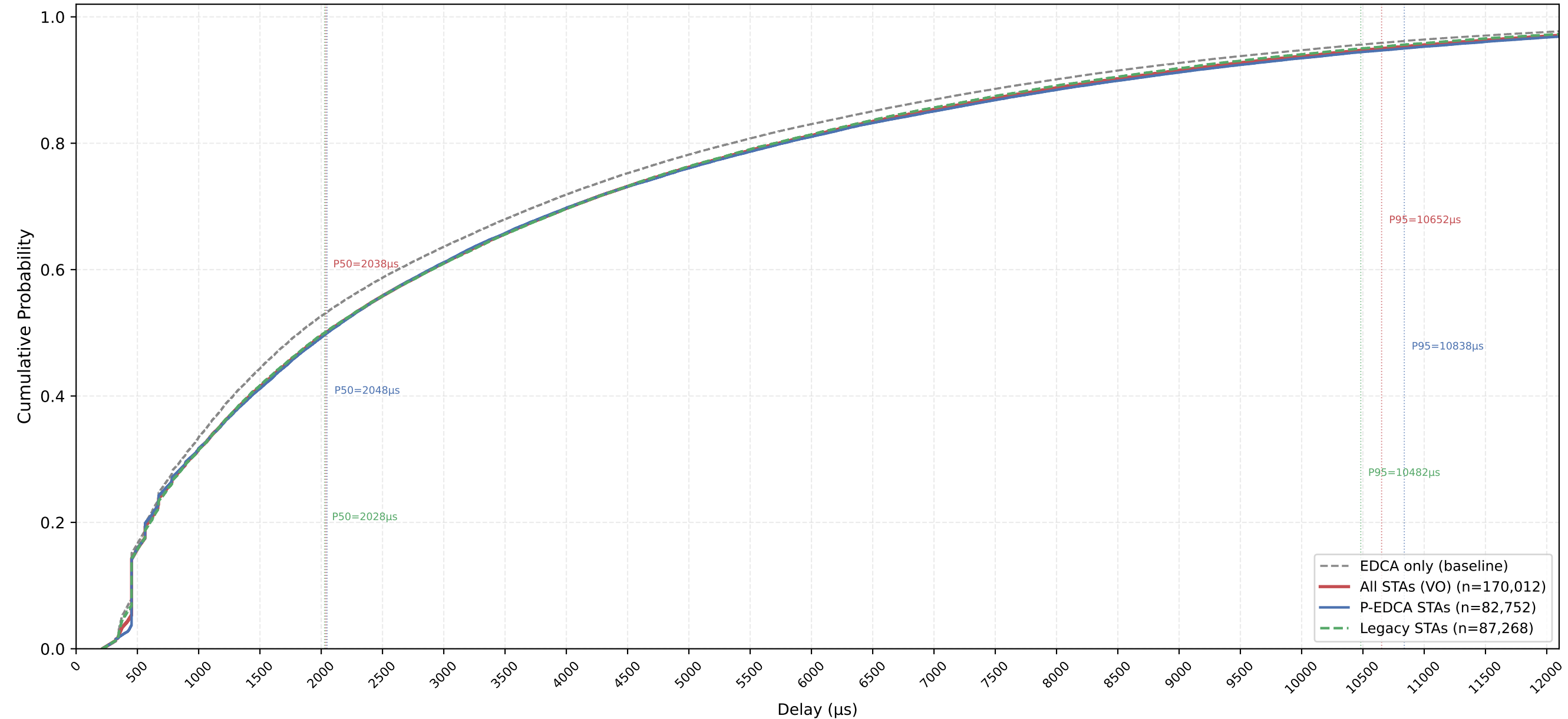
VO Delay CDF — P-EDCA / Legacy / All | CWds=1 × QSRC=0 × PSRC=2 nSta=30, nPedca=15/30, 1Mbps, avg of 10 runs
