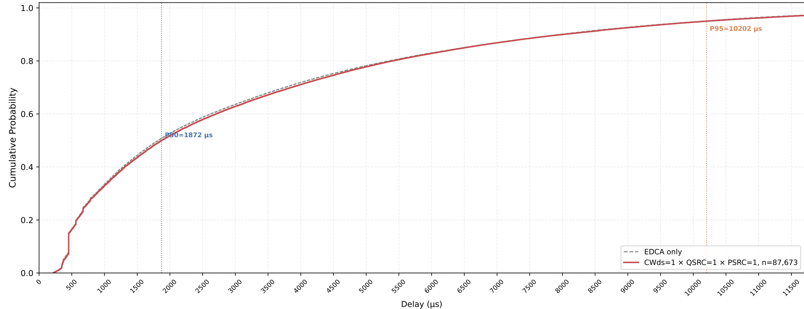
Legacy STA VO Delay CDF — CWds=1 × QSRC=1 × PSRC=1 nSta=30, nPedca=15, 1Mbps, avg of 10 runs
