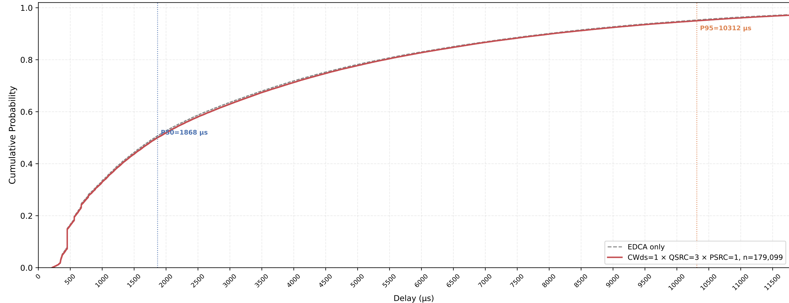
VO (all STAs) Delay CDF — CWds=1 × QSRC=3 × PSRC=1 nSta=30, nPedca=5, 1Mbps, avg of 10 runs
