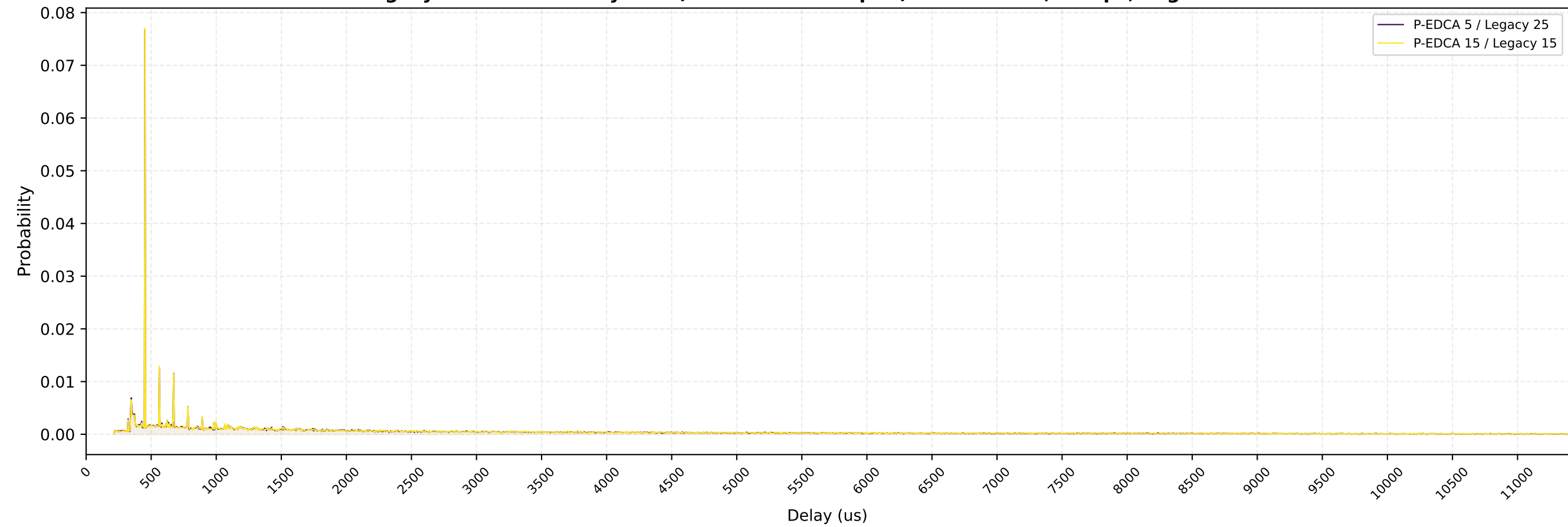
Legacy EDCA STAs Delay PDF (zoomed to 95th pctl) — nSta=30, 1Mbps, avg of 10 runs
