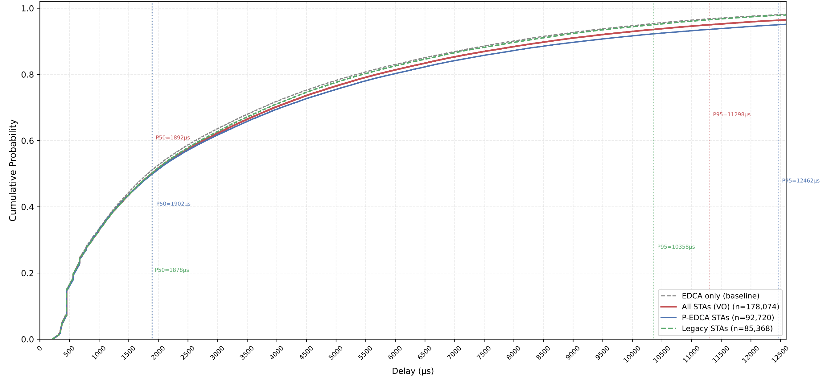
VO Delay CDF — P-EDCA / Legacy / All | CWds=1 × QSRC=4 × PSRC=3 nSta=30, nPedca=15/30, 1Mbps, avg of 10 runs
