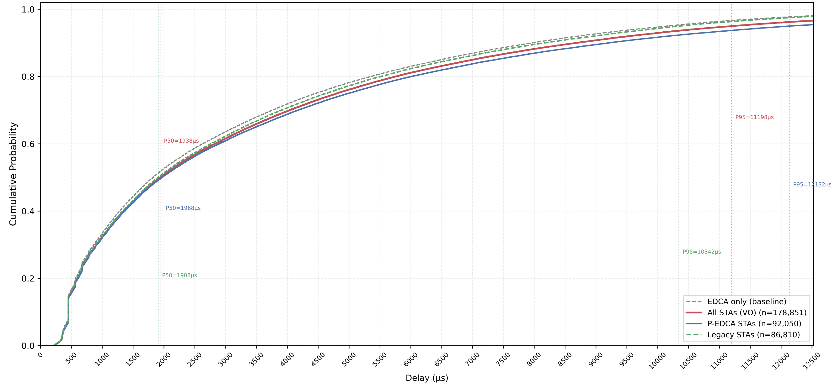
VO Delay CDF — P-EDCA / Legacy / All | CWds=1 × QSRC=5 × PSRC=2 nSta=30, nPedca=15/30, 1Mbps, avg of 10 runs
