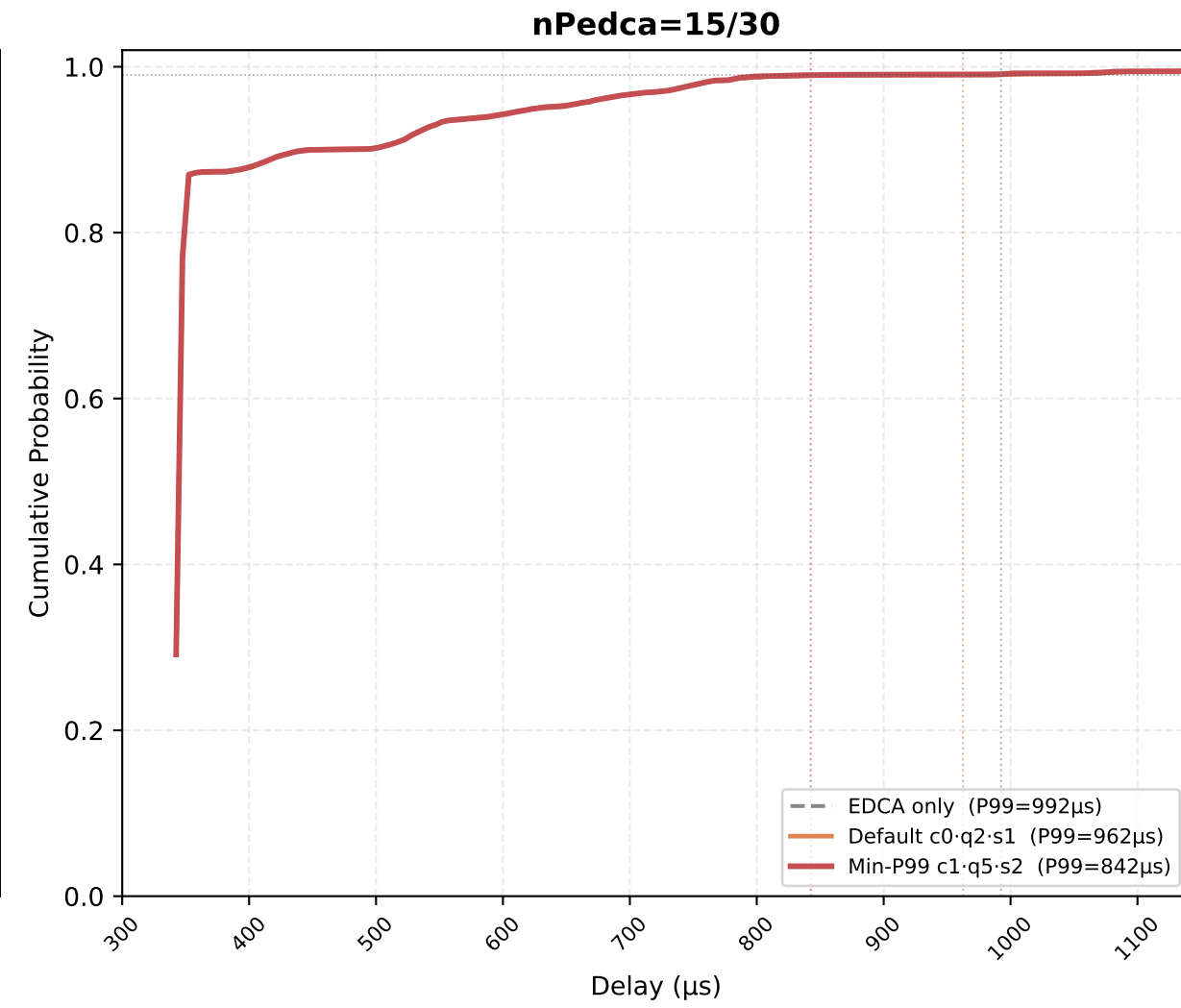
All STAs — Min-P99 vs Default (c0·q2·s1) vs EDCA-only | nSta=30, 0.1Mbps, 10 runs avg
