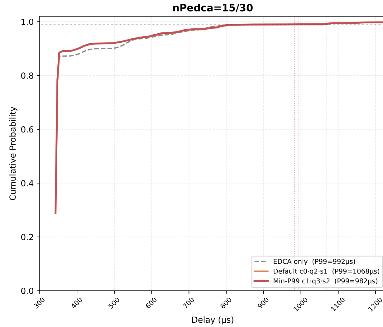
P-EDCA STAs — Min-P99 vs Default (c0·q2·s1) vs EDCA-only | nSta=30, 0.1Mbps, 10 runs avg
