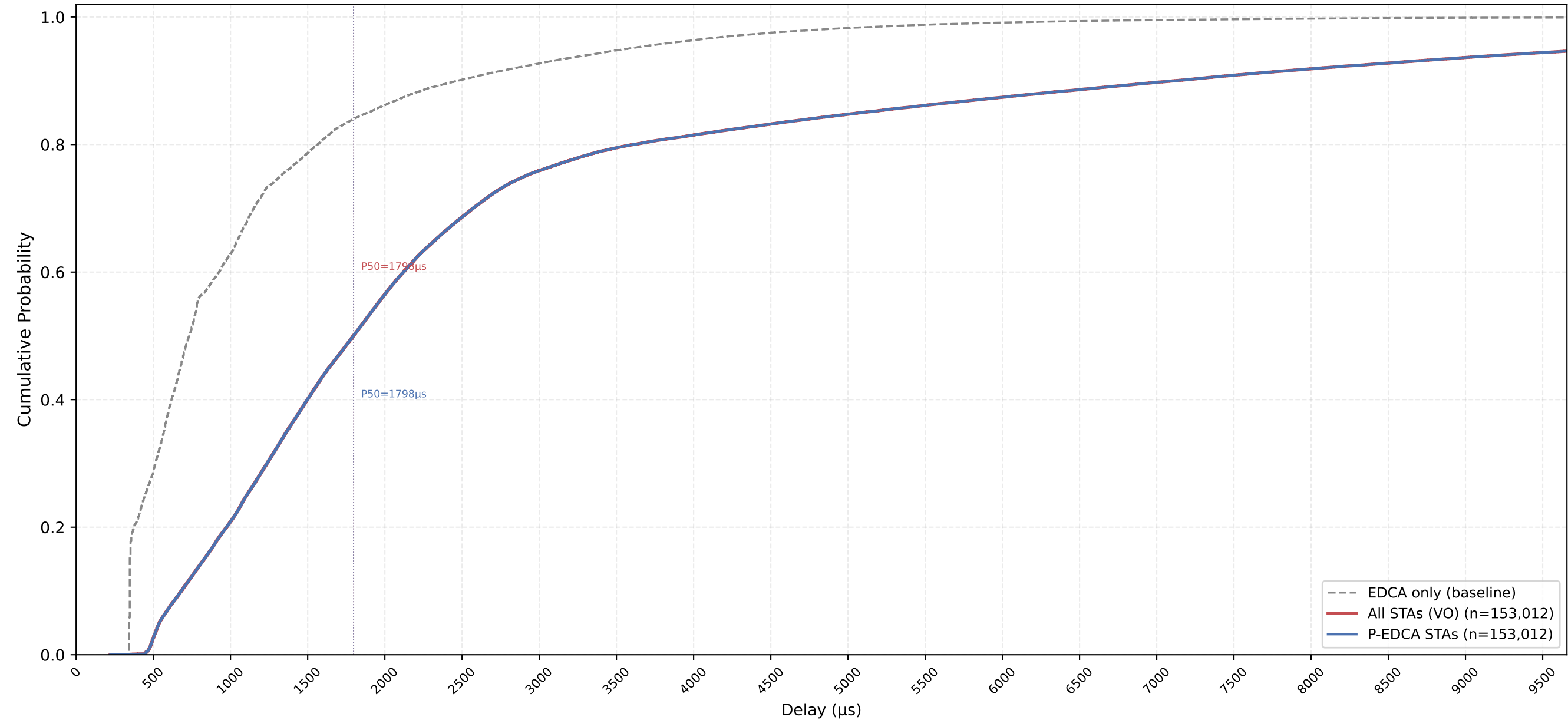
VO Delay CDF — P-EDCA / Legacy / All | CWds=0 × QSRC=0 × PSRC=2 nSta=30, nPedca=30/30, 0.5Mbps, avg of 10 runs
