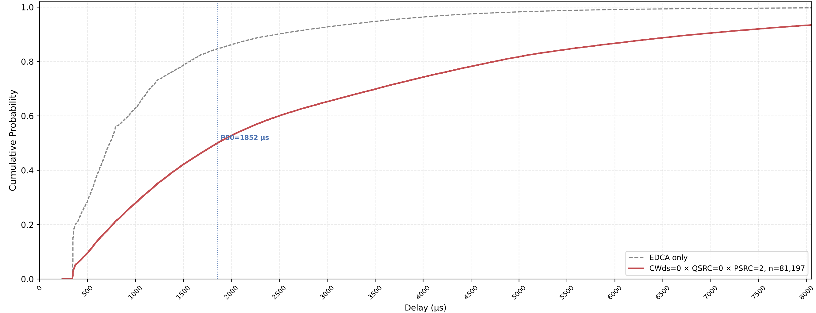
Legacy STA VO Delay CDF — CWds=0 × QSRC=0 × PSRC=2 nSta=30, nPedca=15, 0.5Mbps, avg of 10 runs
