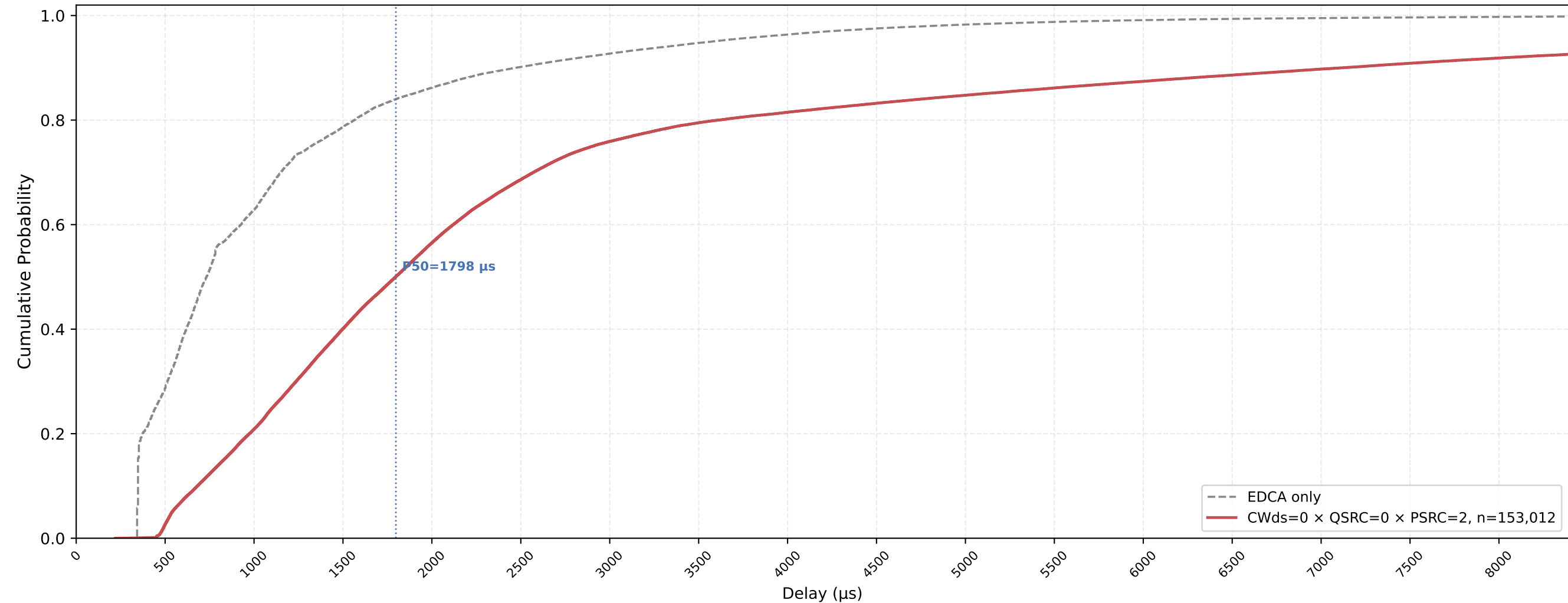
VO (all STAs) Delay CDF — CWds=0 × QSRC=0 × PSRC=2 nSta=30, nPedca=30, 0.5Mbps, avg of 10 runs
