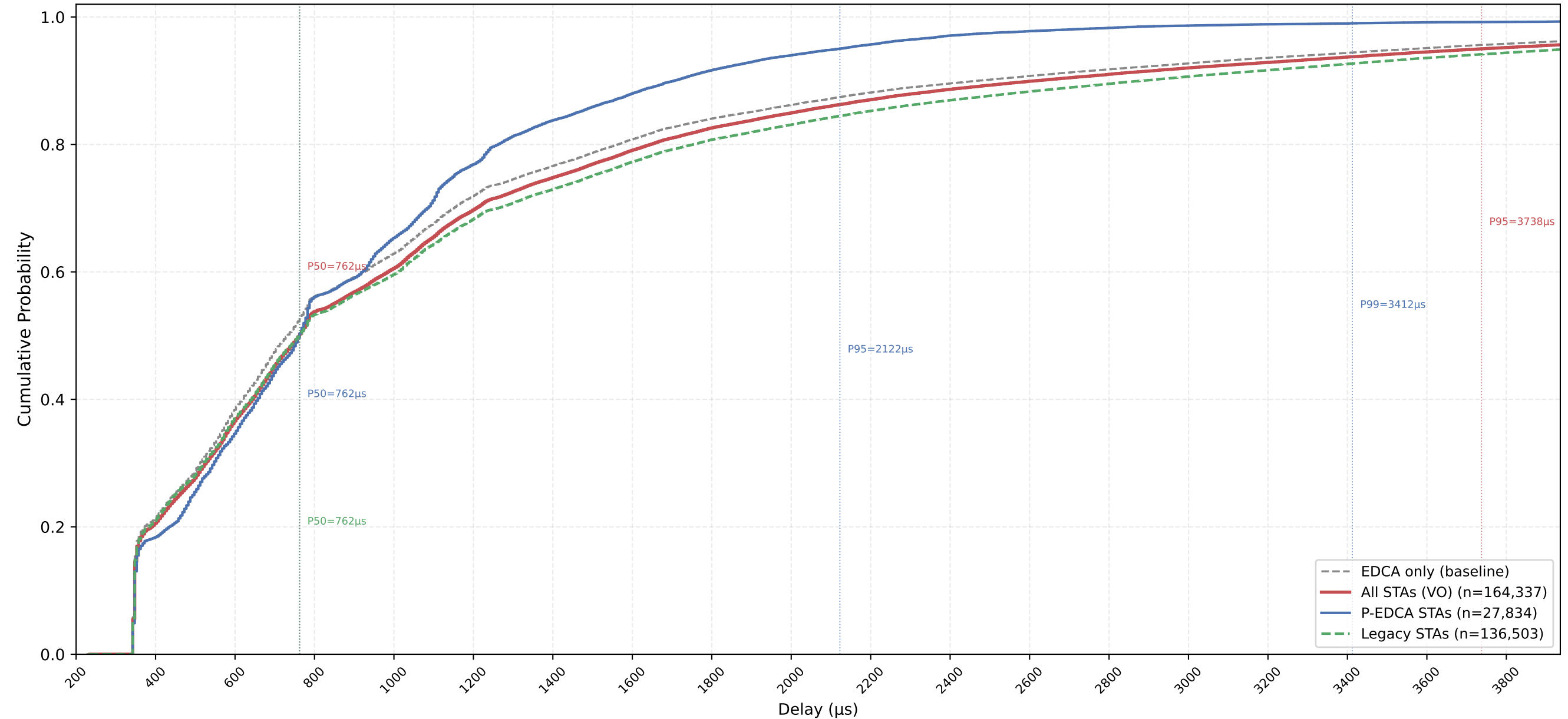
VO Delay CDF — P-EDCA / Legacy / All | CWds=0 × QSRC=1 × PSRC=2 nSta=30, nPedca=5/30, 0.5Mbps, avg of 10 runs
