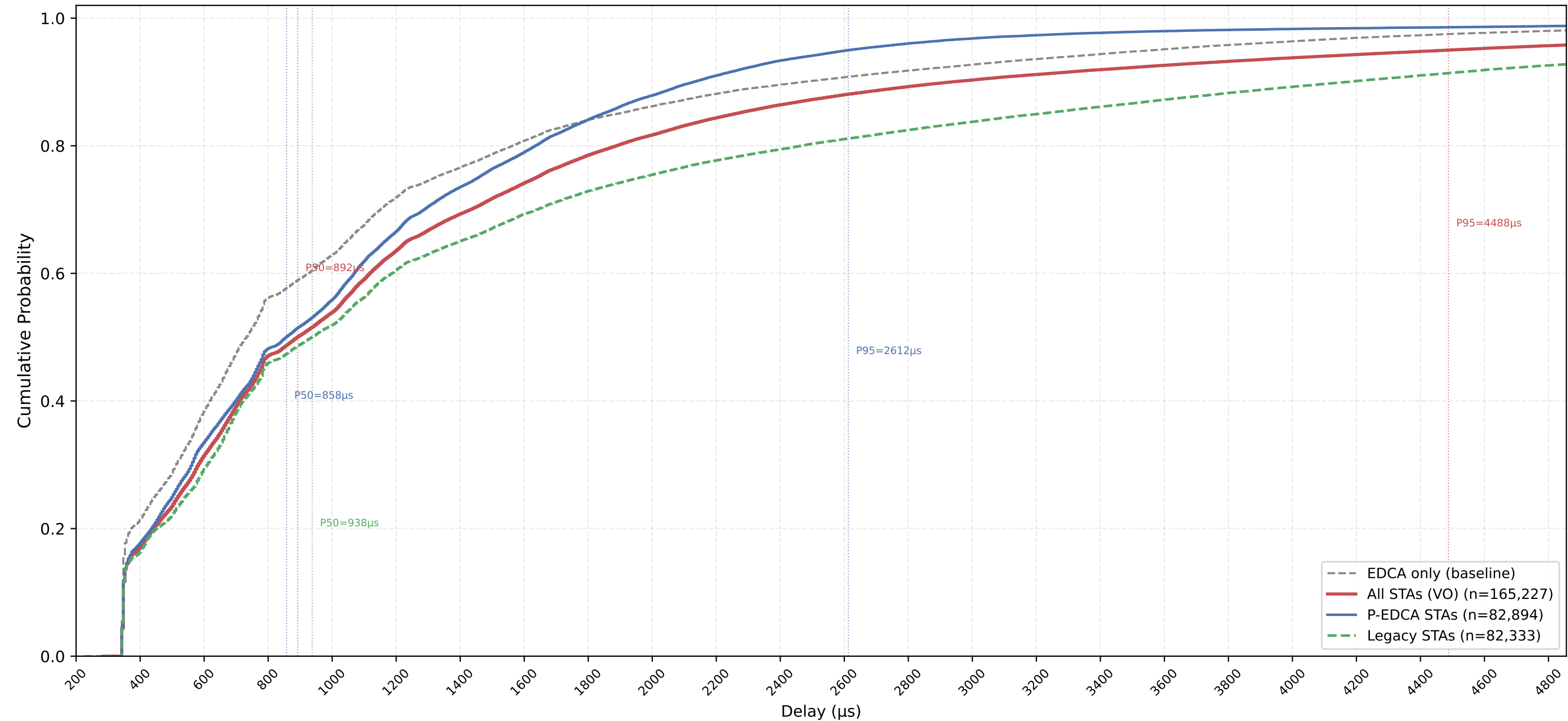
VO Delay CDF — P-EDCA / Legacy / All | CWds=0 × QSRC=1 × PSRC=2 nSta=30, nPedca=15/30, 0.5Mbps, avg of 10 runs
