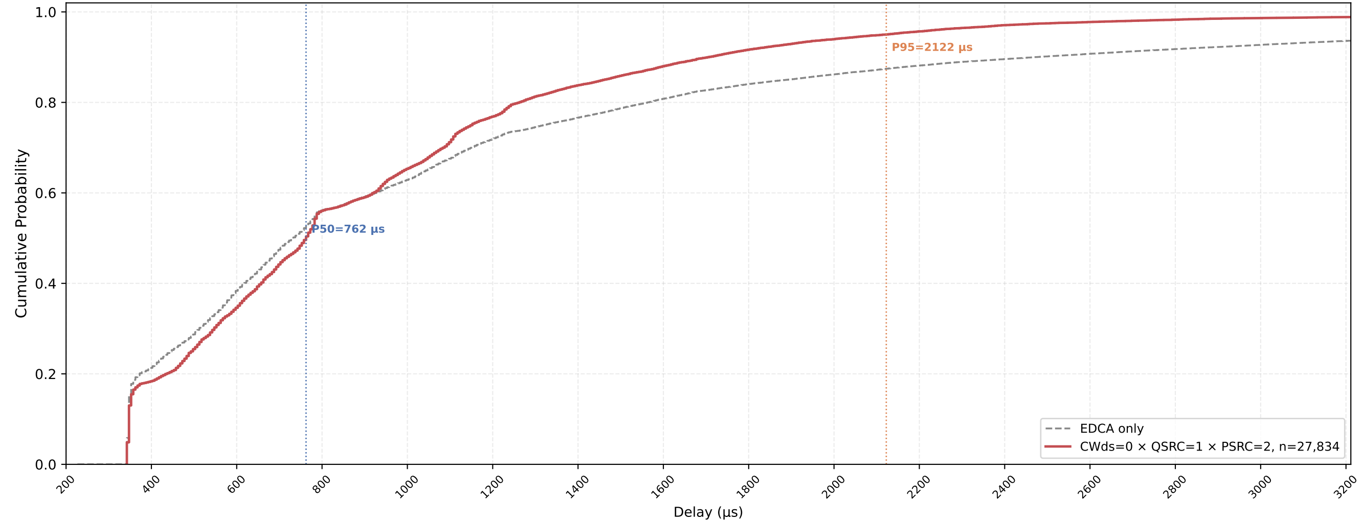
P-EDCA STA VO Delay CDF — CWds=0 × QSRC=1 × PSRC=2 nSta=30, nPedca=5, 0.5Mbps, avg of 10 runs
