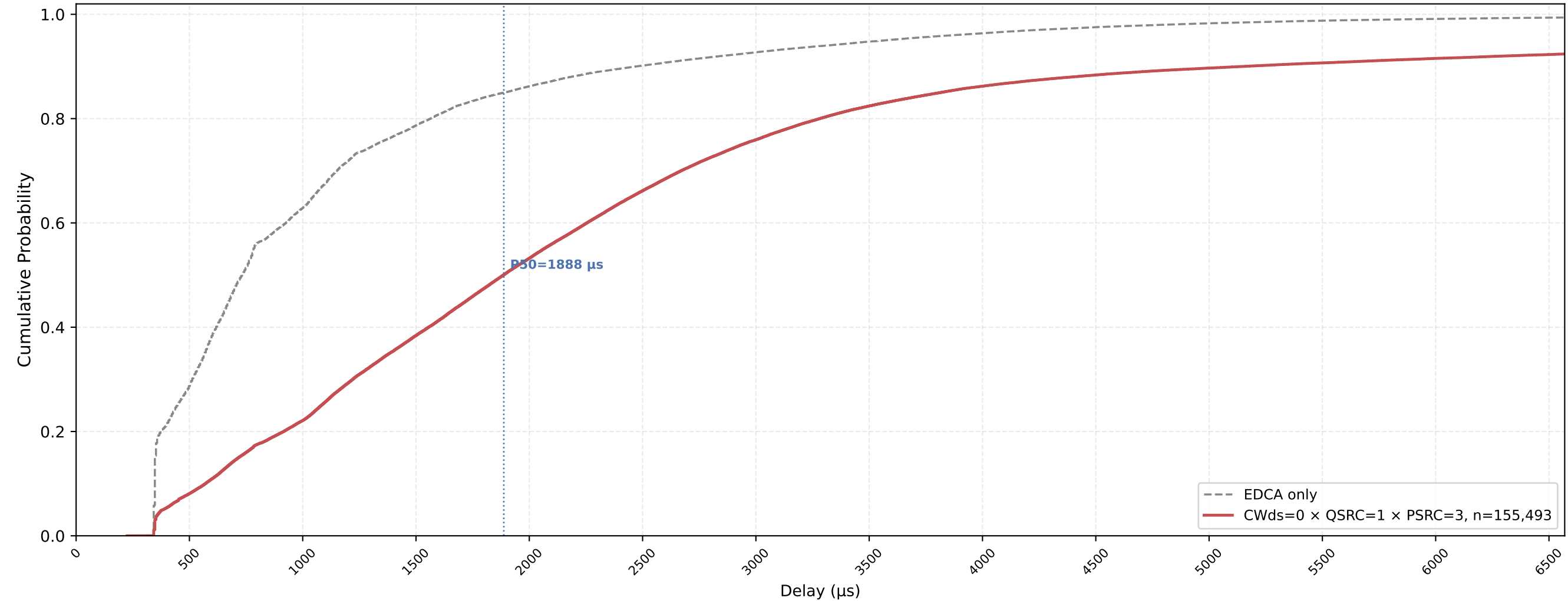
P-EDCA STA VO Delay CDF — CWds=0 × QSRC=1 × PSRC=3 nSta=30, nPedca=30, 0.5Mbps, avg of 10 runs
