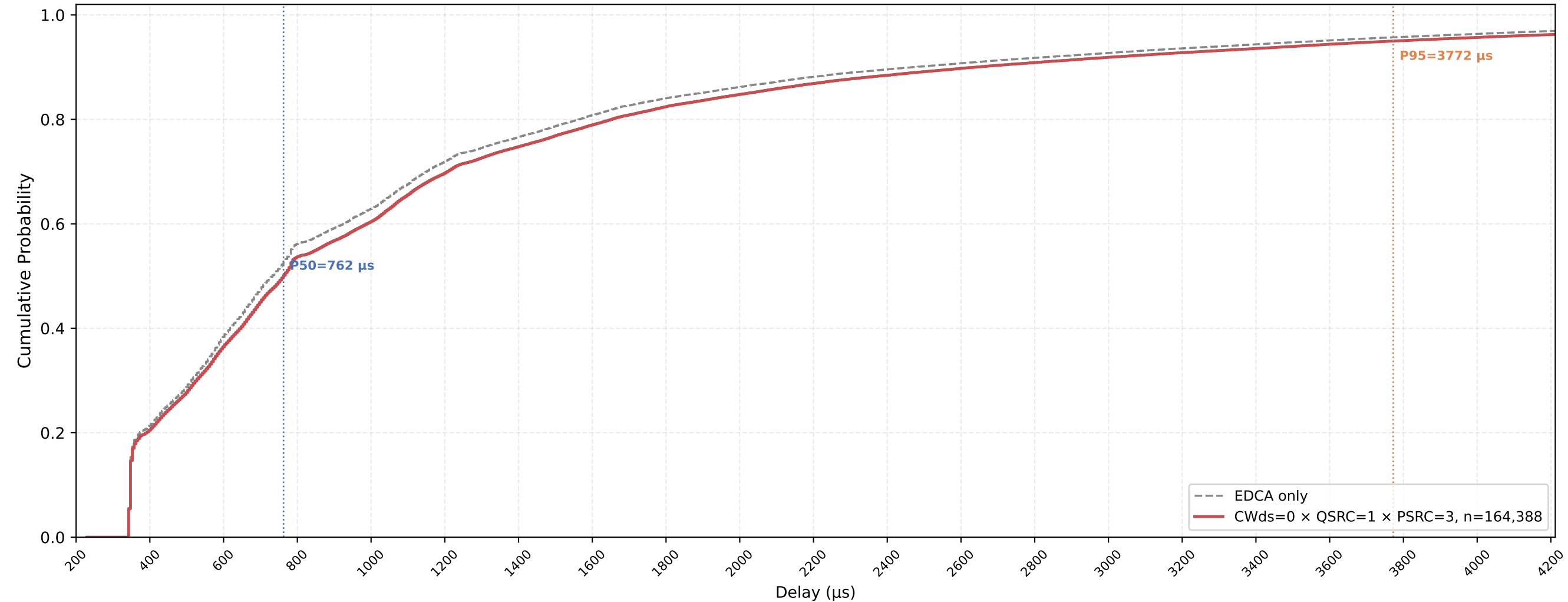
VO (all STAs) Delay CDF — CWds=0 × QSRC=1 × PSRC=3 nSta=30, nPedca=5, 0.5Mbps, avg of 10 runs
