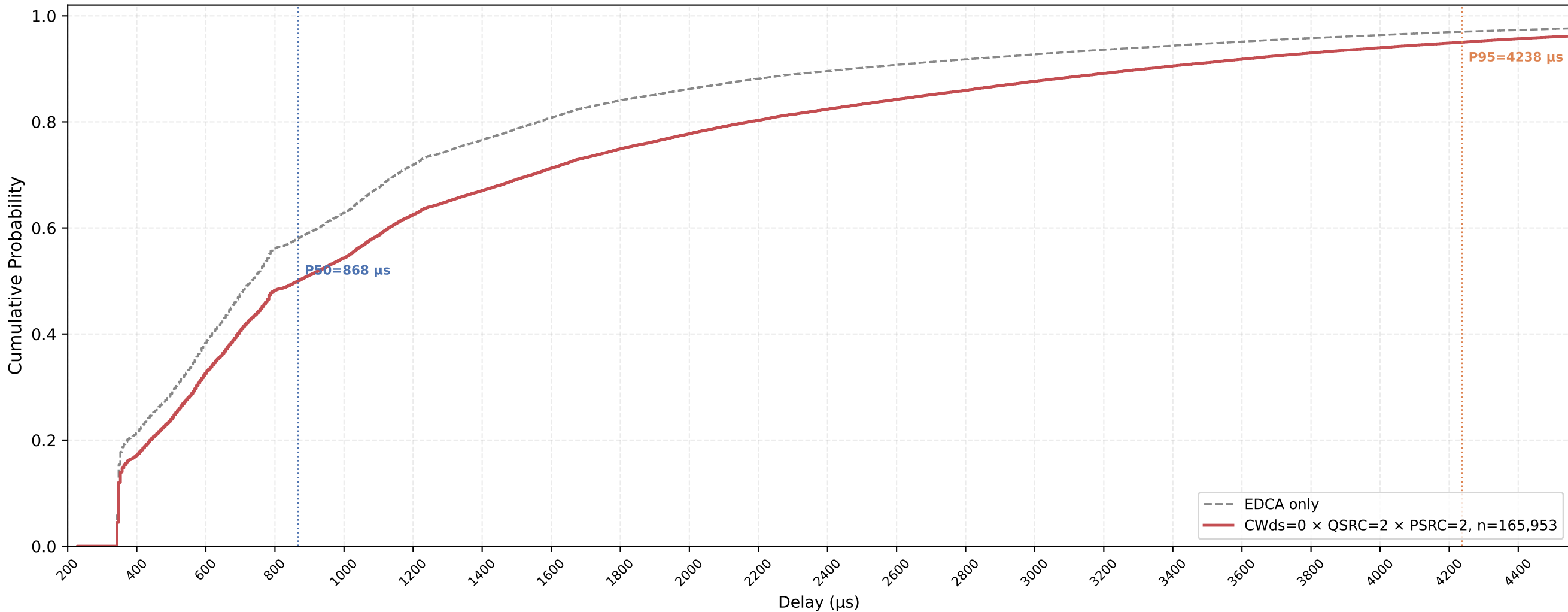
VO (all STAs) Delay CDF — CWds=0 × QSRC=2 × PSRC=2 nSta=30, nPedca=30, 0.5Mbps, avg of 10 runs
