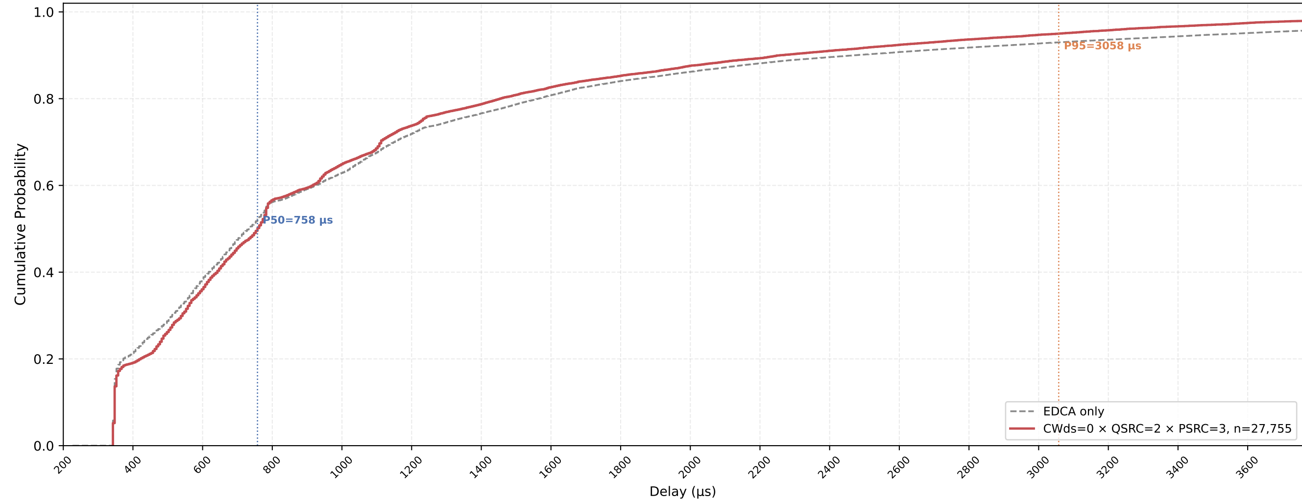
P-EDCA STA VO Delay CDF — CWds=0 × QSRC=2 × PSRC=3 nSta=30, nPedca=5, 0.5Mbps, avg of 10 runs
