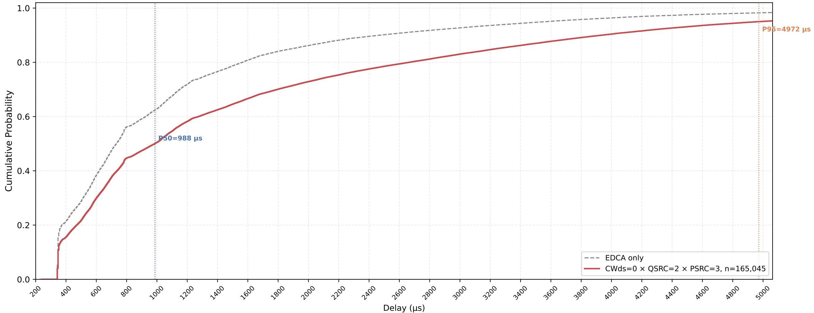
P-EDCA STA VO Delay CDF — CWds=0 × QSRC=2 × PSRC=3 nSta=30, nPedca=30, 0.5Mbps, avg of 10 runs
