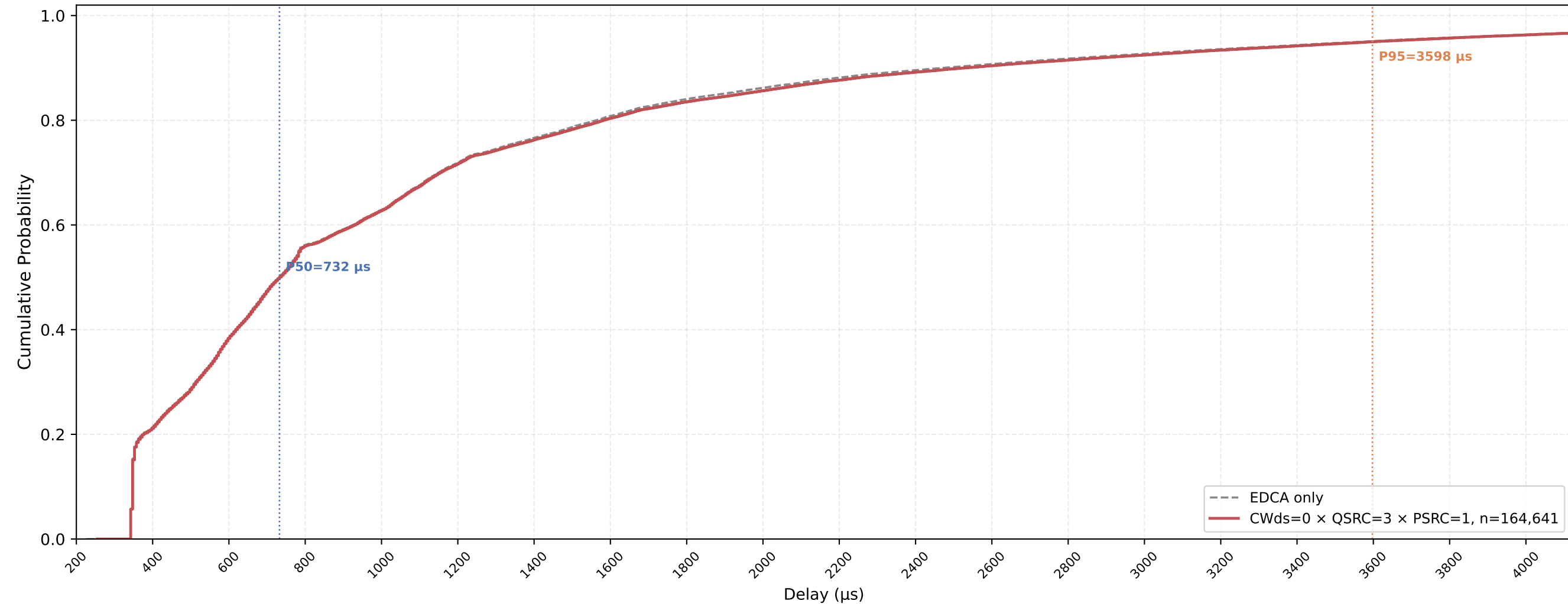
VO (all STAs) Delay CDF — CWds=0 × QSRC=3 × PSRC=1 nSta=30, nPedca=5, 0.5Mbps, avg of 10 runs
