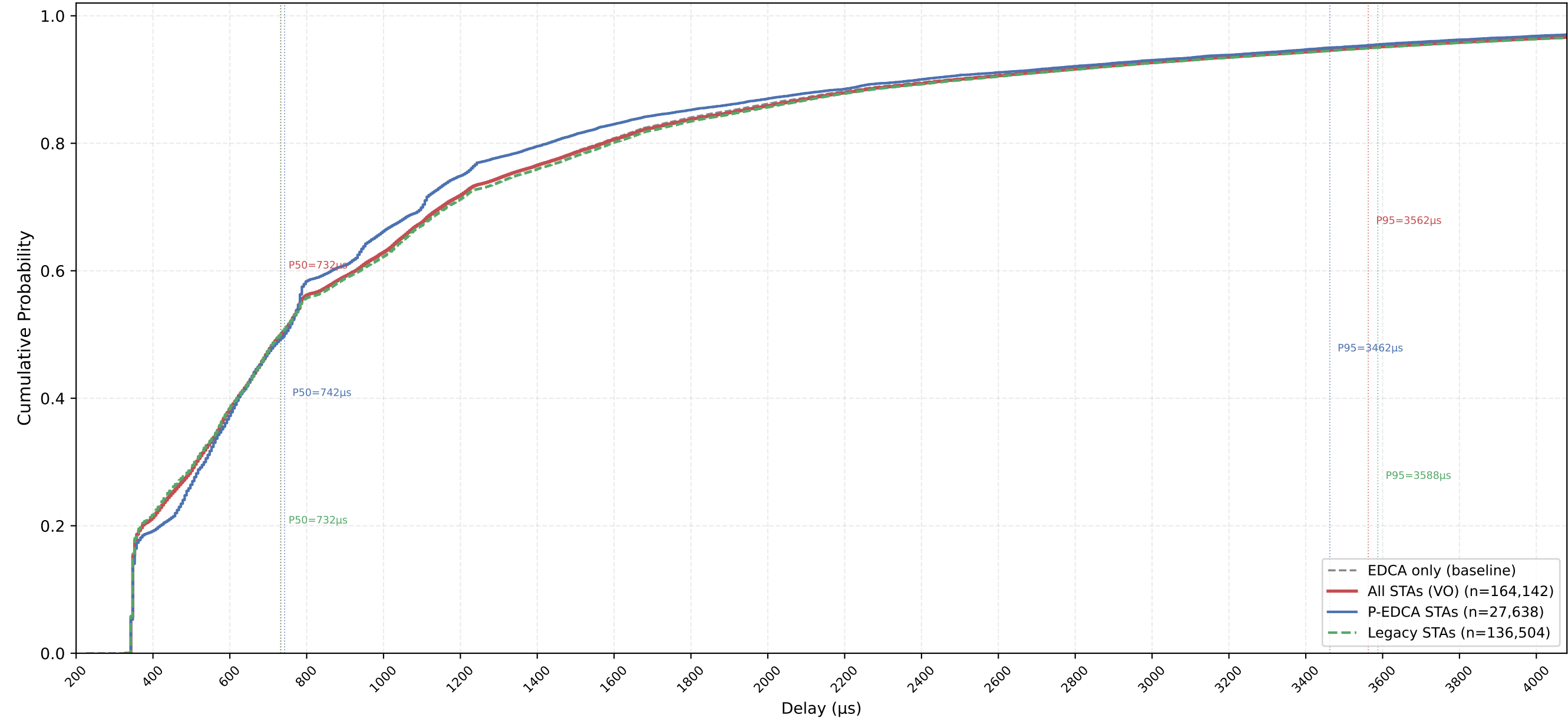
VO Delay CDF — P-EDCA / Legacy / All | CWds=0 × QSRC=3 × PSRC=2 nSta=30, nPedca=5/30, 0.5Mbps, avg of 10 runs
