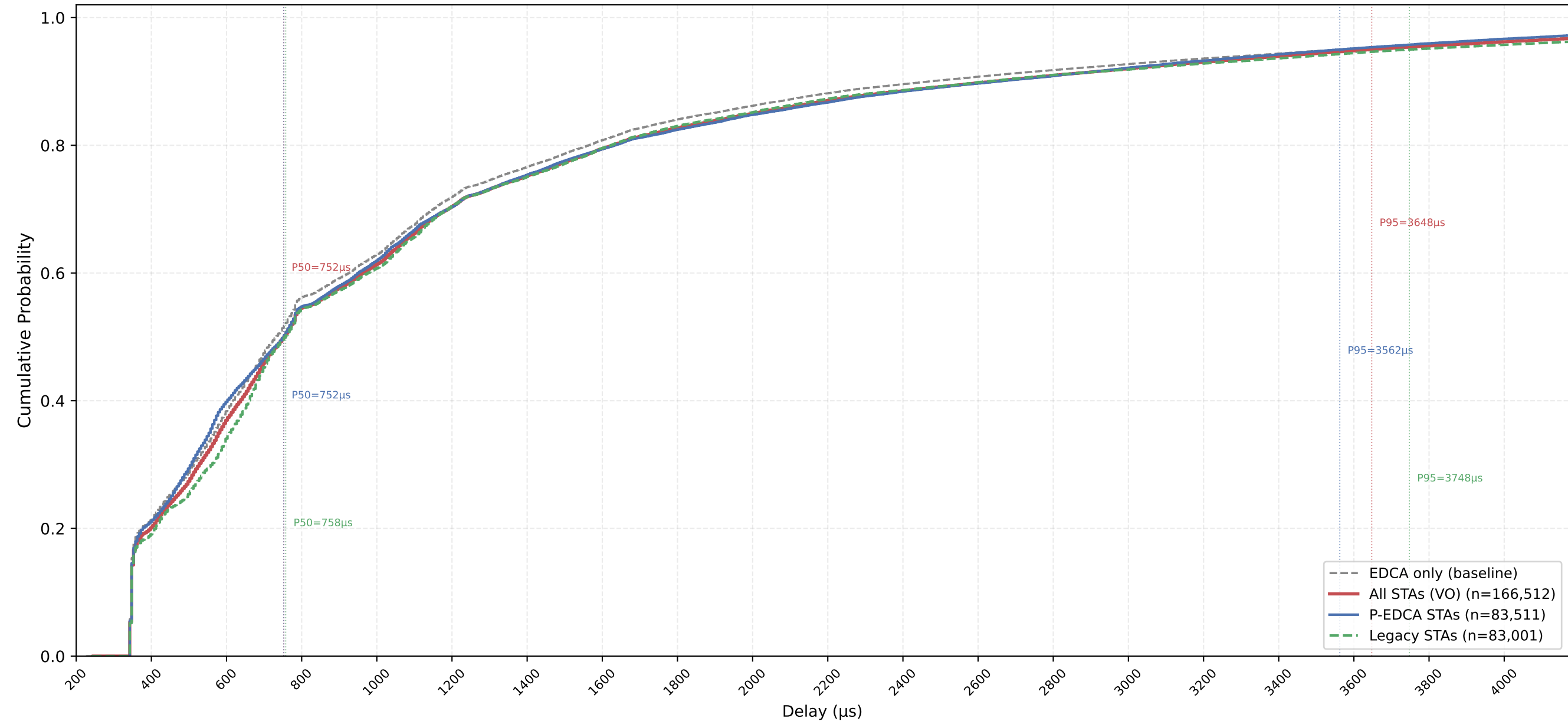
VO Delay CDF — P-EDCA / Legacy / All | CWds=0 × QSRC=3 × PSRC=2 nSta=30, nPedca=15/30, 0.5Mbps, avg of 10 runs
