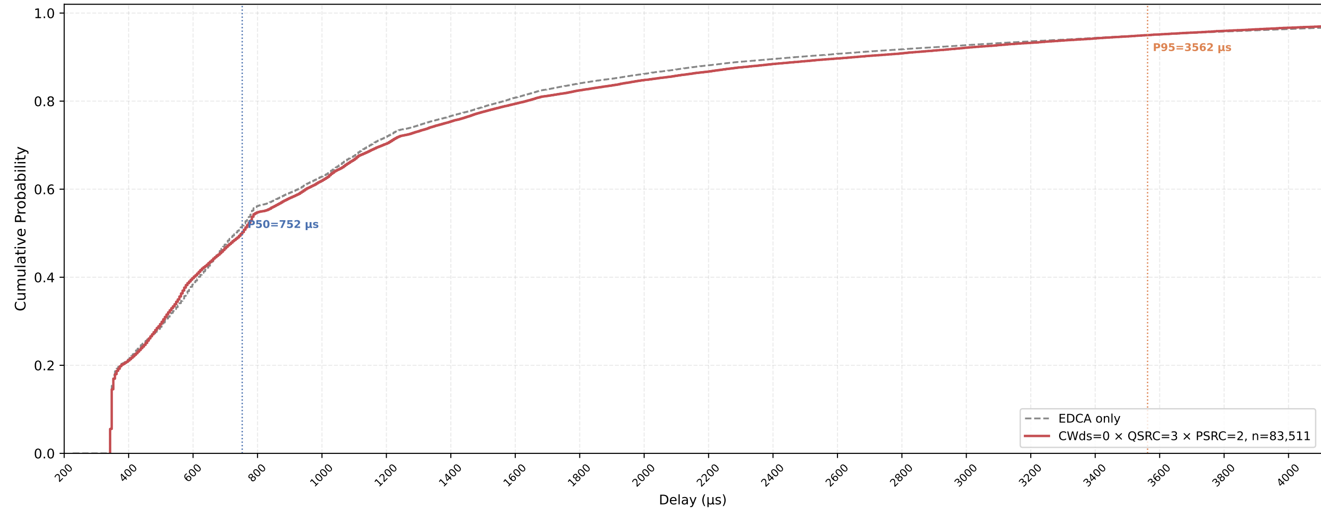
P-EDCA STA VO Delay CDF — CWds=0 × QSRC=3 × PSRC=2 nSta=30, nPedca=15, 0.5Mbps, avg of 10 runs
