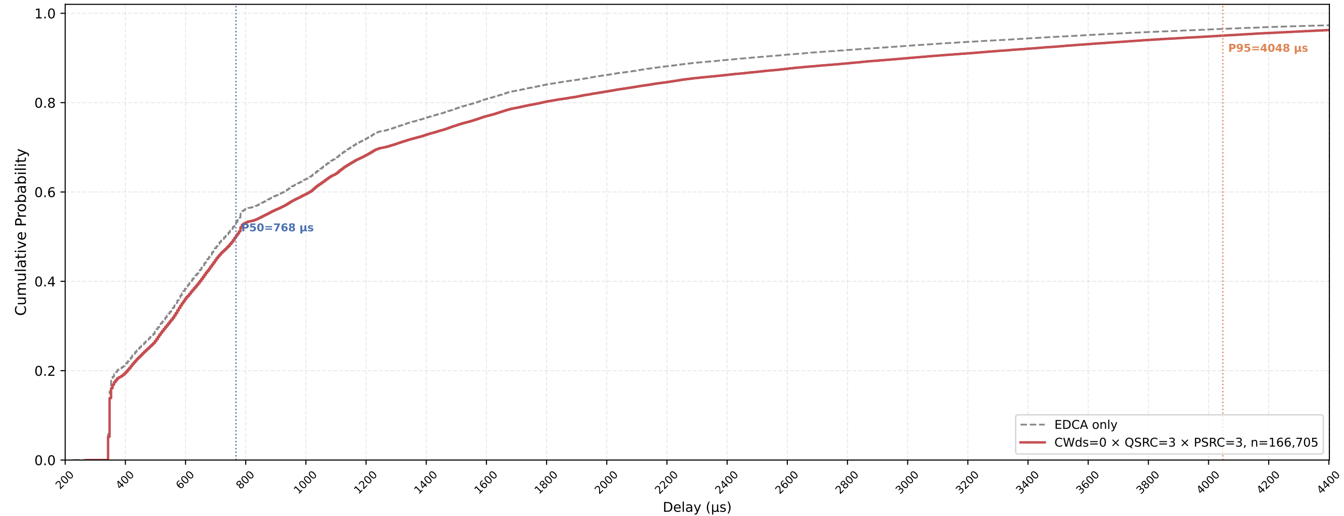
P-EDCA STA VO Delay CDF — CWds=0 × QSRC=3 × PSRC=3 nSta=30, nPedca=30, 0.5Mbps, avg of 10 runs
